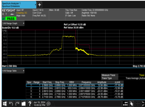
B2_N41(20M)_DFT-s- OFDM_BPSK_Outer_Full_High_CH
