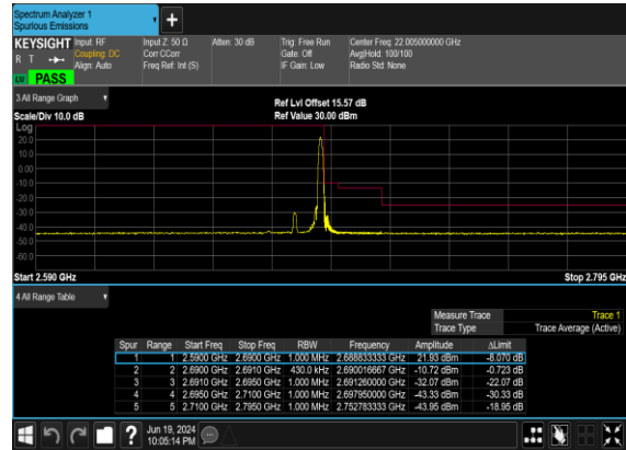
B2_N41(20M)_DFT-s- OFDM_QPSK_Edge_1RB_Right_High_CH
