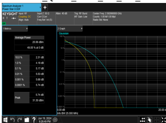
B2_N41(20M)_DFT-s-OFDM_QPSK_Outer_Full_Mid_CH
