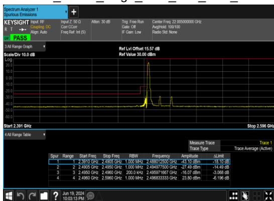
B2_N41(20M)_DFT-s- OFDM_BPSK_Edge_1RB_Left_Low_CH
