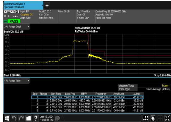
B2_N41(20M)_DFT-s- OFDM_QPSK_Outer_Full_High_CH
