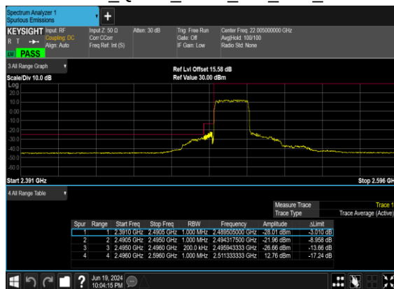
B2_N41(20M)_DFT-s- OFDM_QPSK_Outer_Full_Low_CH
