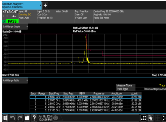
B2_N41(20M)_DFT-s- OFDM_BPSK_Edge_1RB_Right_High_CH
