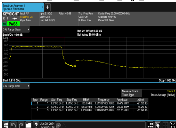
B48_N25(5M)_DFT-s- OFDM_BPSK_Outer_Full_High_CH
