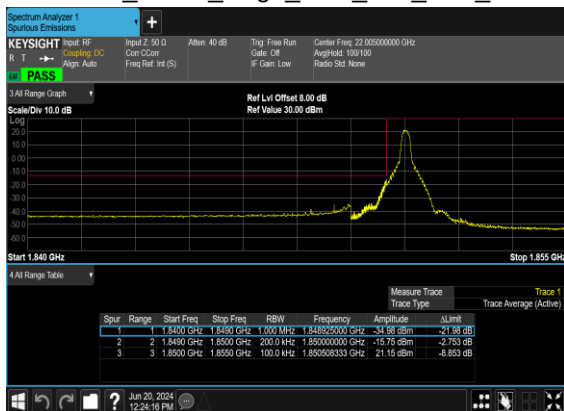
B48_N25(20M)_DFT-s- OFDM_BPSK_Edge_1RB_Left_Low_CH
