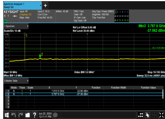
B48_N25(5M)_DFT-s- OFDM_QPSK_Edge_1RB_Left_High_CH
