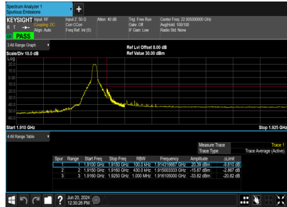
B48_N25(40M)_DFT-s- OFDM_QPSK_Edge_1RB_Right_High_CH
