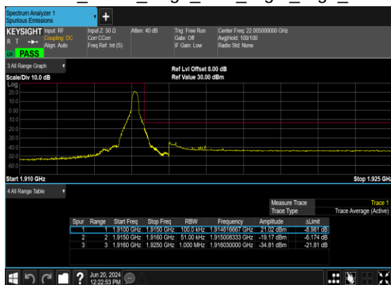
B48_N25(5M)_DFT-s- OFDM_BPSK_Edge_1RB_Right_High_CH
