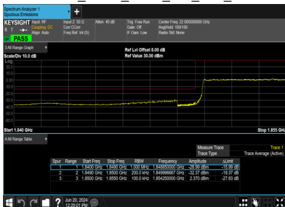
B48_N25(20M)_DFT-s- OFDM_BPSK_Outer_Full_Low_CH
