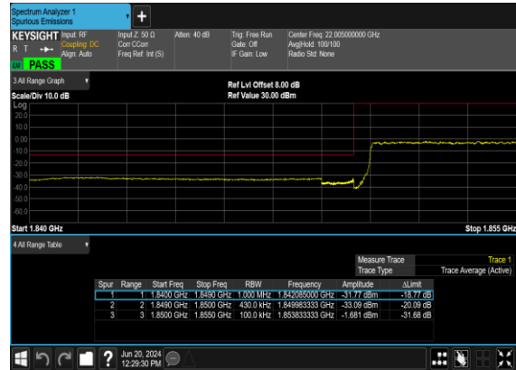
B48_N25(40M)_DFT-s- OFDM_QPSK_Outer_Full_Low_CH
