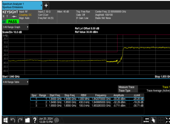
B48_N25(40M)_DFT-s- OFDM_BPSK_Outer_Full_Low_CH
