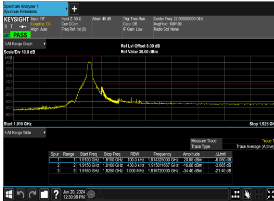
B48_N25(40M)_DFT-s- OFDM_BPSK_Edge_1RB_Right_High_CH
