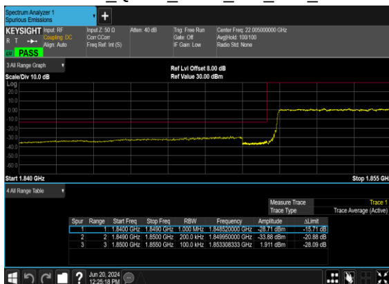
B48_N25(20M)_DFT-s- OFDM_QPSK_Outer_Full_Low_CH
