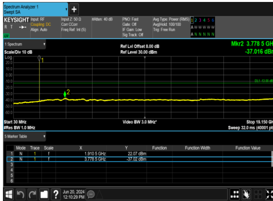
B48_N25(5M)_DFT-s- OFDM_BPSK_Edge_1RB_Left_High_CH
