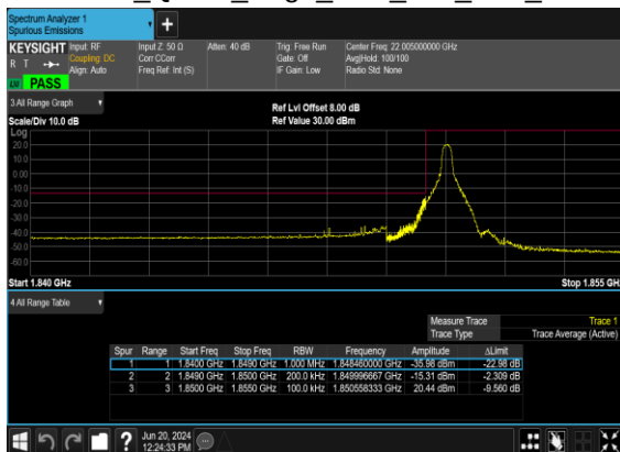
B48_N25(20M)_DFT-s- OFDM_QPSK_Edge_1RB_Left_Low_CH
