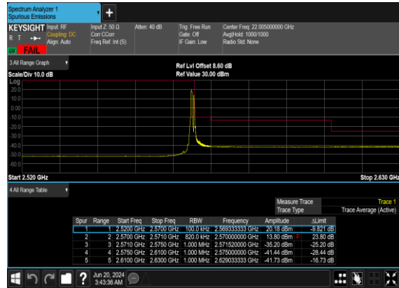
B2_N7(40M)_DFT-s- OFDM_BPSK_Edge_1RB_Right_High_CH
