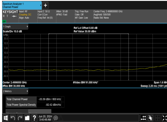
B2_N7(40M)_DFT-s- OFDM_QPSK_Outer_Full_Low_CH_CHP_PASS
