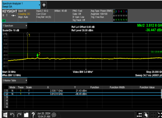
B5_N7(40M)_DFT-s- OFDM_QPSK_Edge_1RB_Left_High_CH
