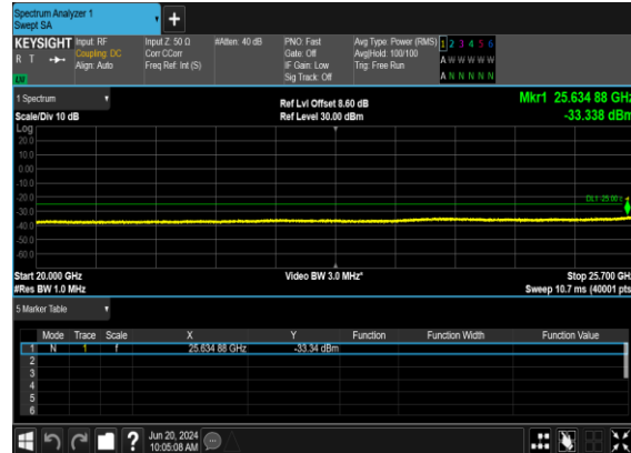
B5_N7(40M)_DFT-s- OFDM_QPSK_Edge_1RB_Left_High_CH
