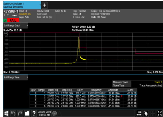
B2_N7(40M)_DFT-s- OFDM_QPSK_Edge_1RB_Right_High_CH
