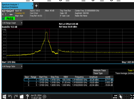
B12_N25(5M)_DFT-s- OFDM_QPSK_Edge_1RB_Right_High_CH
