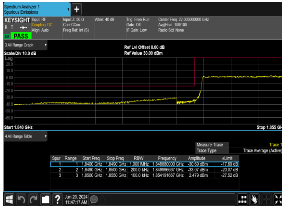
B12_N25(20M)_DFT-s- OFDM_BPSK_Outer_Full_Low_CH
