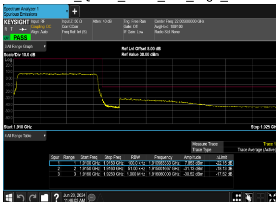
B12_N25(5M)_DFT-s- OFDM_QPSK_Outer_Full_High_CH
