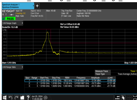
B12_N25(5M)_DFT-s- OFDM_BPSK_Edge_1RB_Right_High_CH
