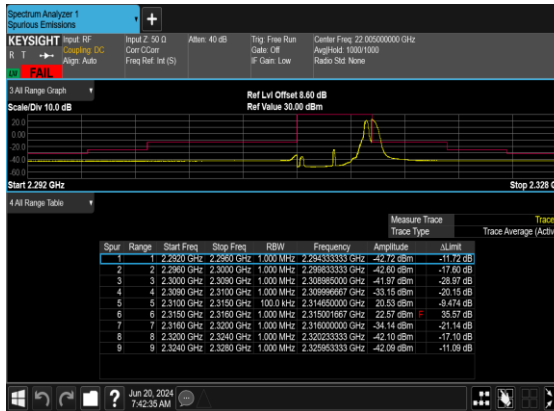
B5_N30(5M)_DFT-s- OFDM_QPSK_Edge_1RB_Right_High_CH
