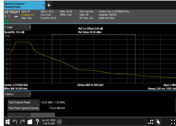
B5_N30(5M)_DFT-s- OFDM_QPSK_Edge_1RB_Right_High_CH_CHP_P ASS
