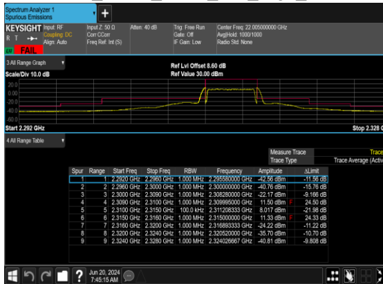
B5_N30(5M)_DFT-s- OFDM_BPSK_Outer_Full_High_CH
