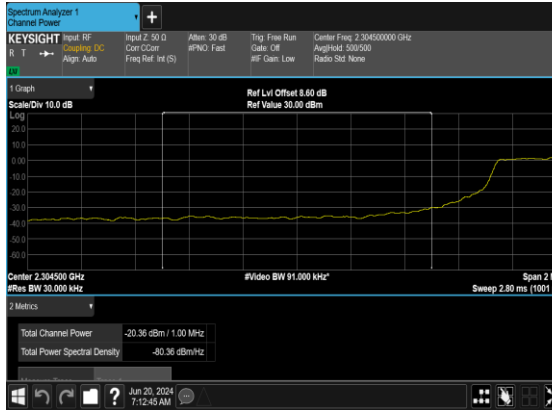
B5_N30(5M)_DFT-s- OFDM_QPSK_Outer_Full_Low_CH_CH_P SS
