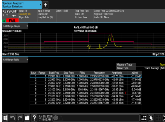
B5_N30(5M)_DFT-s- OFDM_BPSK_Edge_1RB_Right_High_CH
