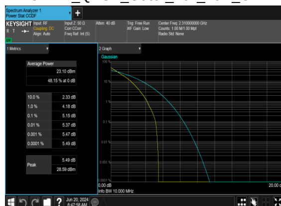
B5_N30(10M)_DFT-s- OFDM QPSK Outer Full Low CH
