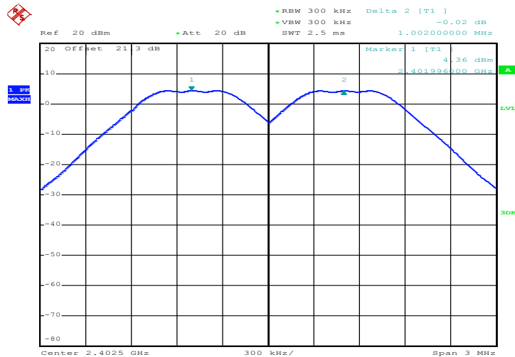
Channel Separation Plot on Channel 00 - 01
