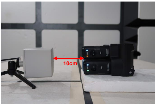
The Field Probe is placed 10cm distance to the front surface of EUT
