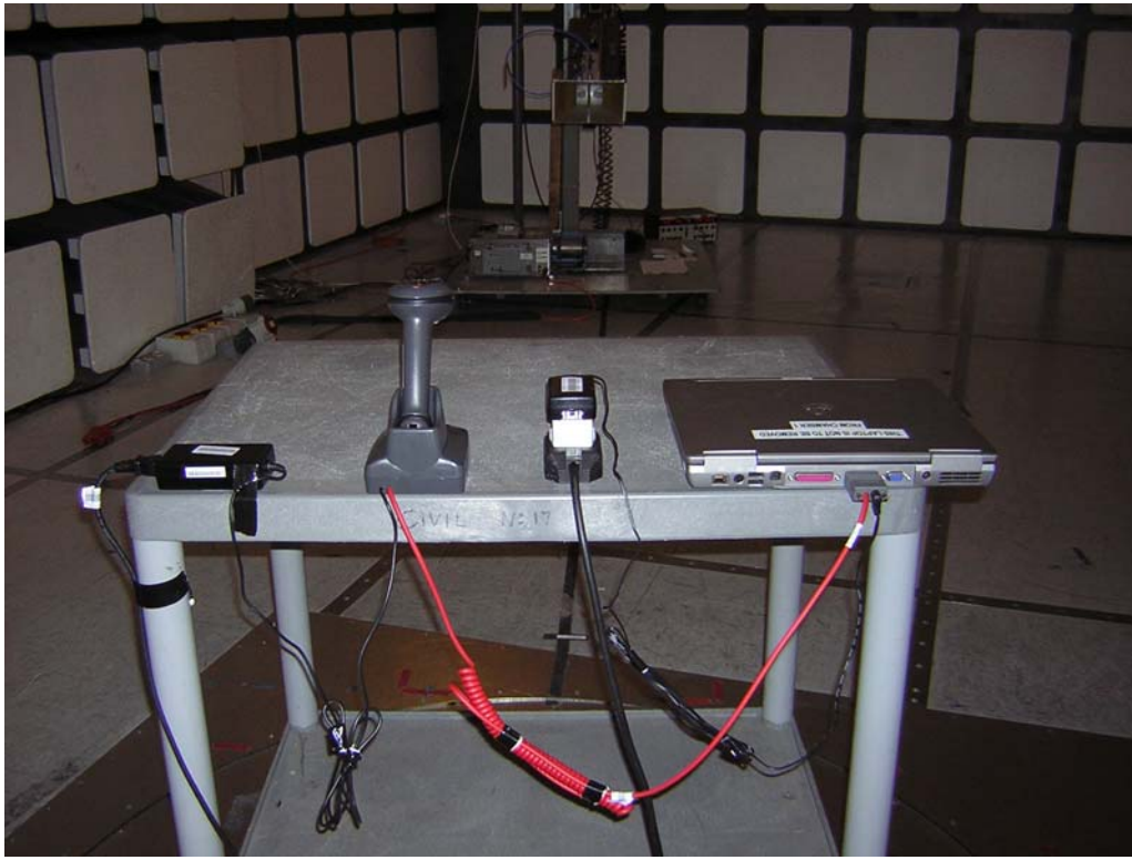
Config 2 – RS232 Radiated Emissions (Enclosure)
