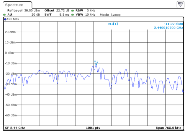
Power Density (dBm/3kHz) Plot Channel 19
