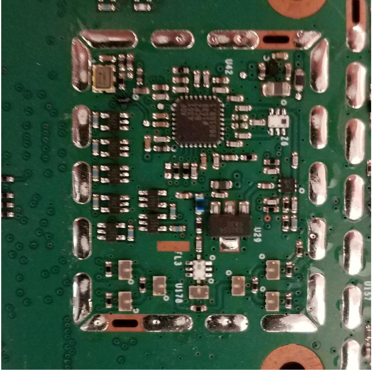
Pcb with shield removed, see page 5 for shield on.
