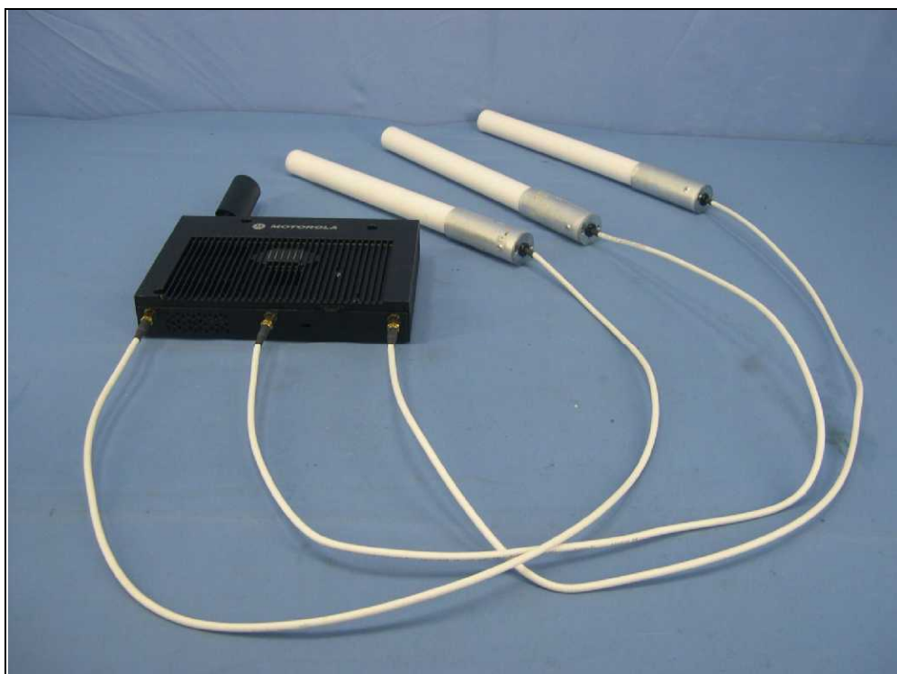
Antenna 7: ML-5299-HPA1-01R
