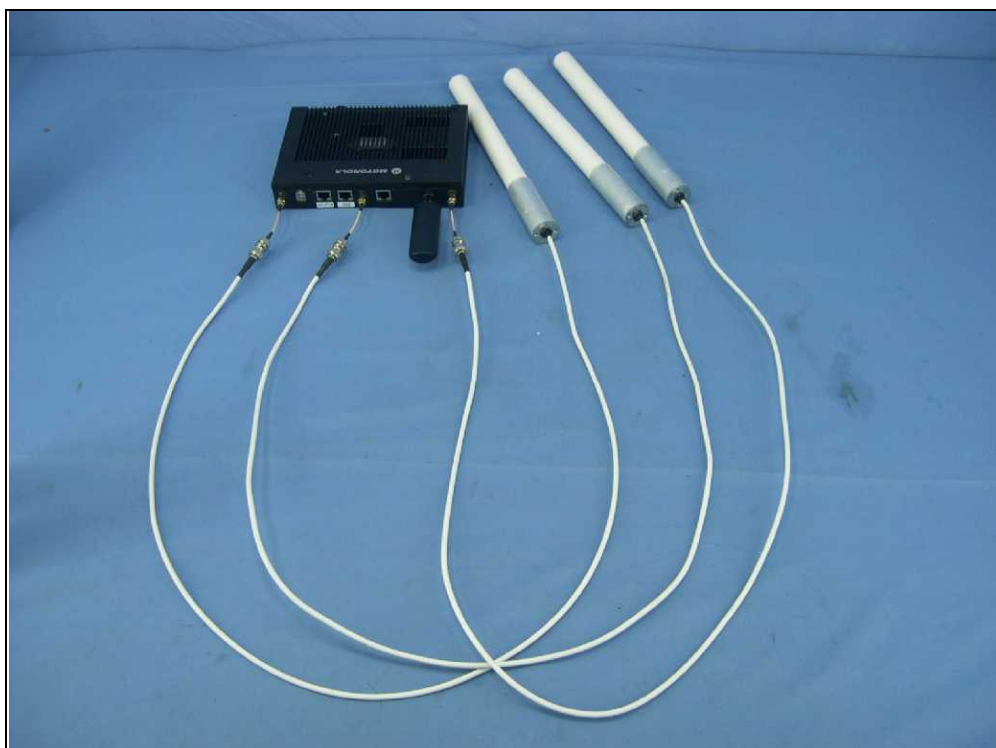
Antenna 6: ML-2499-HPA3-01R
