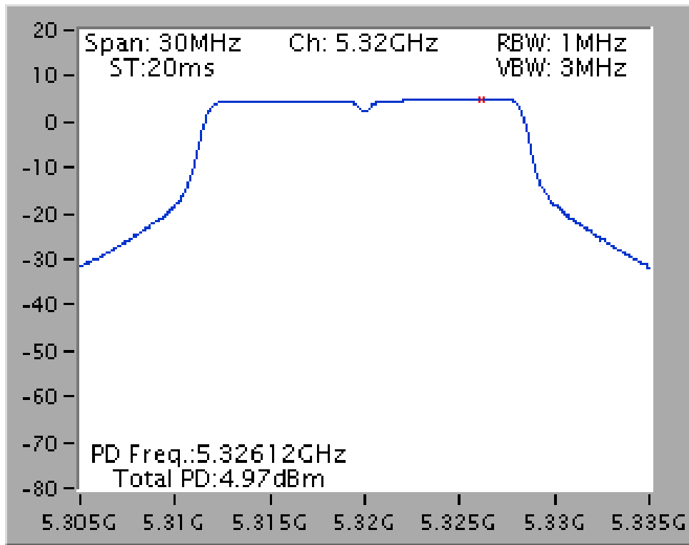
Power Density Plot on Configuration IEEE 802.11a / 2TX / 5320 MHz
