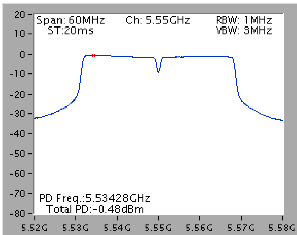
Power Density Plot on Configuration IEEE 802.11n MCS0 40MHz / 2TX / 5550 MHz
