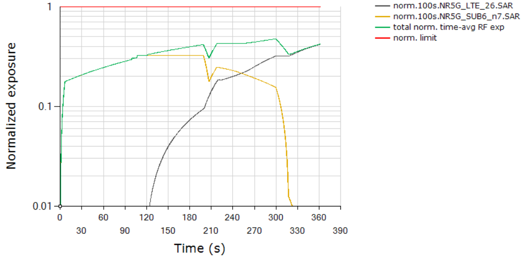
Total Normalized Time-averaged RF Exposure Tech: NR5G LTE, Band 26 / Tech: NR5G SUB6, Band n7
