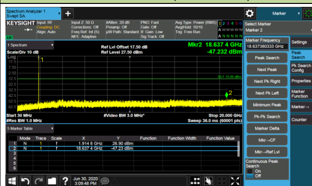
Channel 26675 (1913.5MHz)
