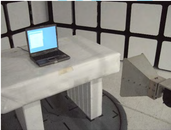
Test Configuration 1: 960 MHz to 40 GHz
