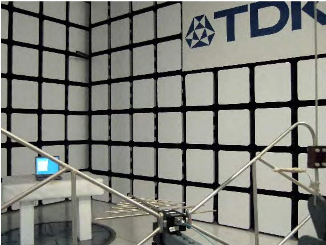
Test Configuration 2: 30 MHz to 960 MHz
