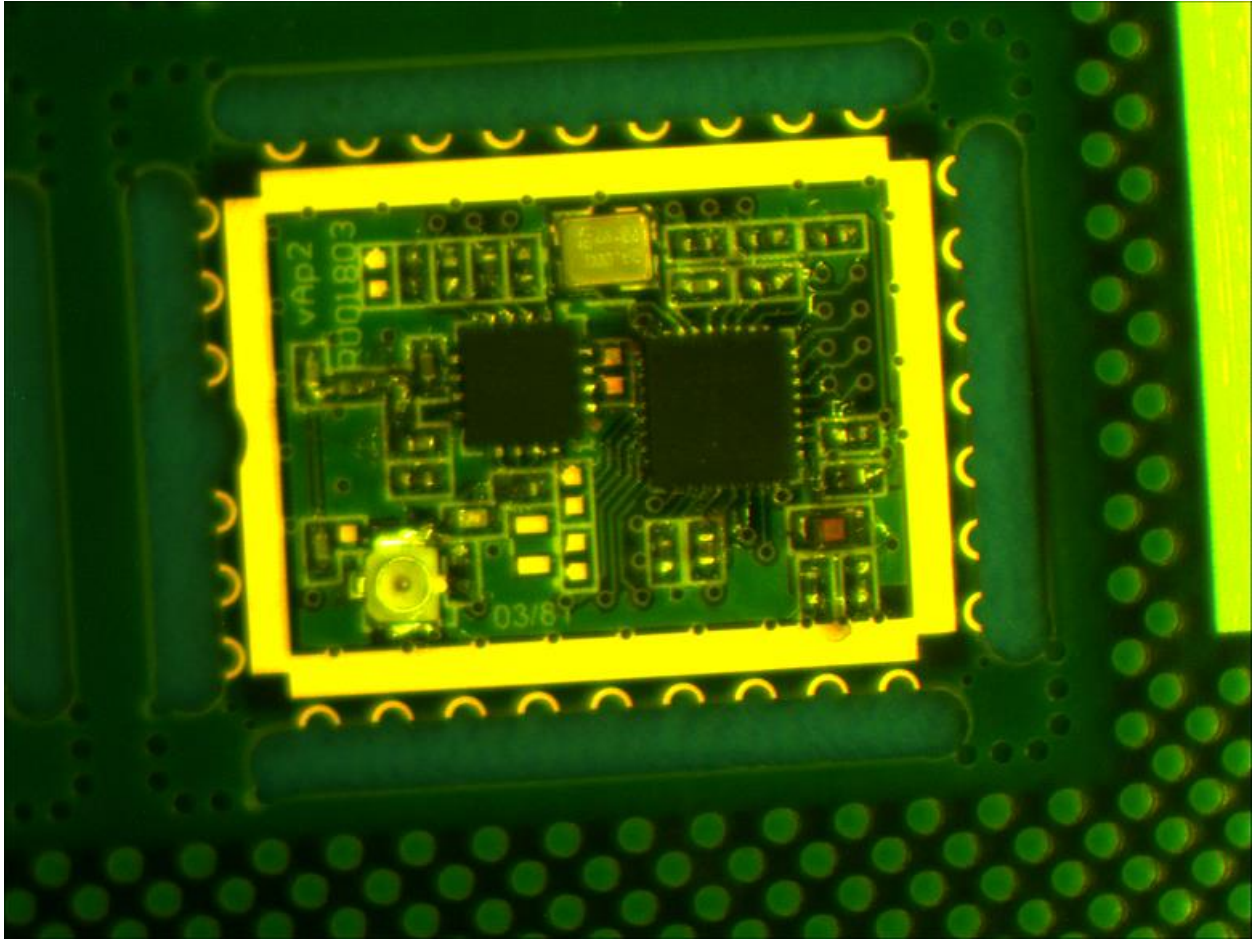
Payload Module Top without Shield
