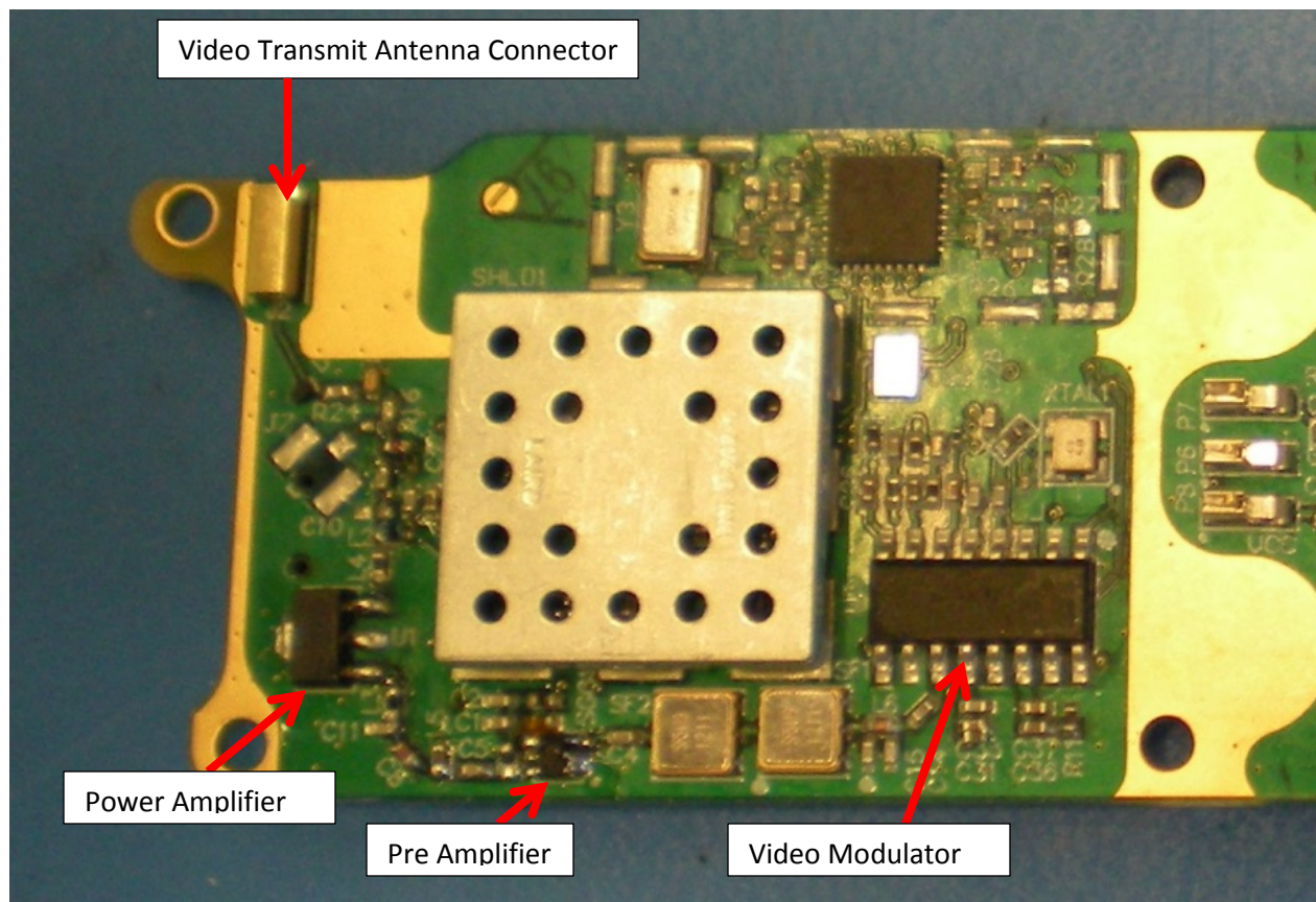
Figure 4: Main Board, Front (annotated functionality)
