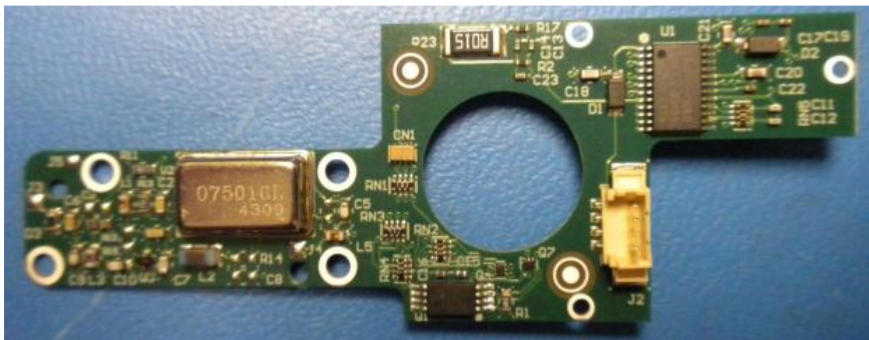
Figure 7: FrontBoard (Top)
