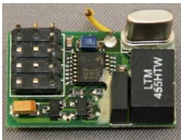
Figure 9: Command Receiver (COTS Product, Top)
