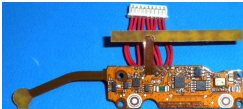
Figure 3: Blister (Top)
