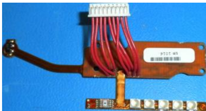
Figure 4: Blister (Bottom)
