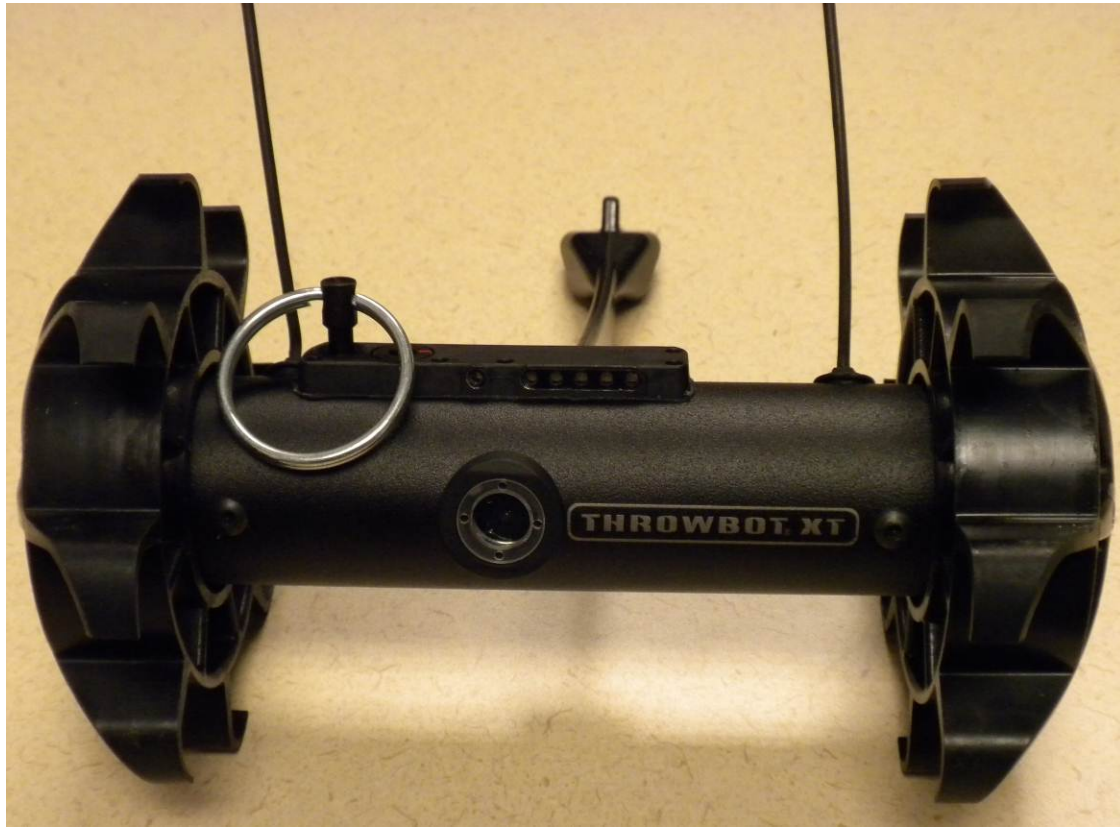
Figure 1: Front View
