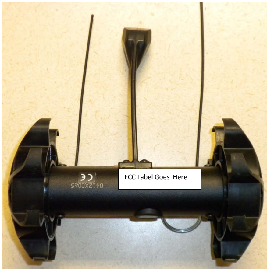
Figure 3: Bottom View
