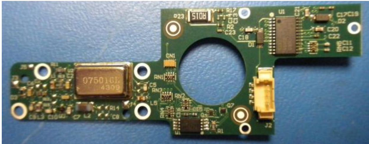
Figure 7: FrontBoard (Top)
