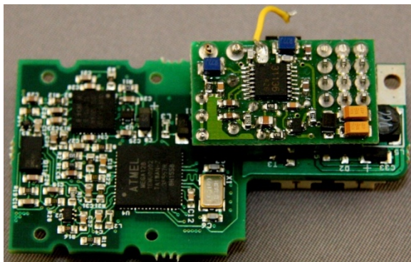
Figure 12: Gyro Board stacked with COTS Command Receiver
