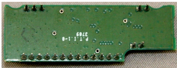
Figure 4: DC-DC Board (Bottom)
