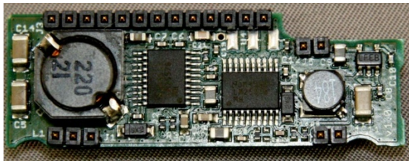
Figure 3: DC-DC Board (Top)
