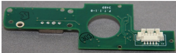
Figure 7: FrontBoard (Bottom)
