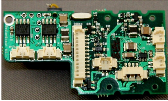
Figure 10: Gyro Board (Top)
