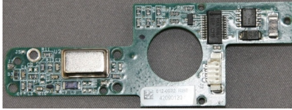
Figure 6: FrontBoard (Top)
