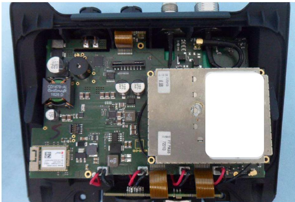
7. PCB Top View
