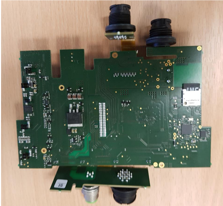
8. PCB Bottom View
