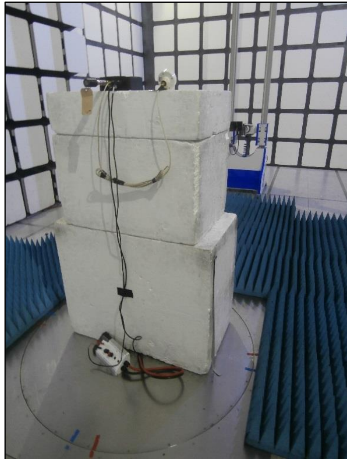
Figure 54 –1 GHz to 2 GHz, EUT Orientation X
