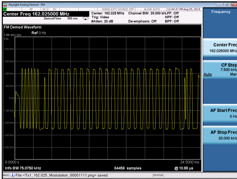
Figure 41- 162.025 MHz - 00001111
