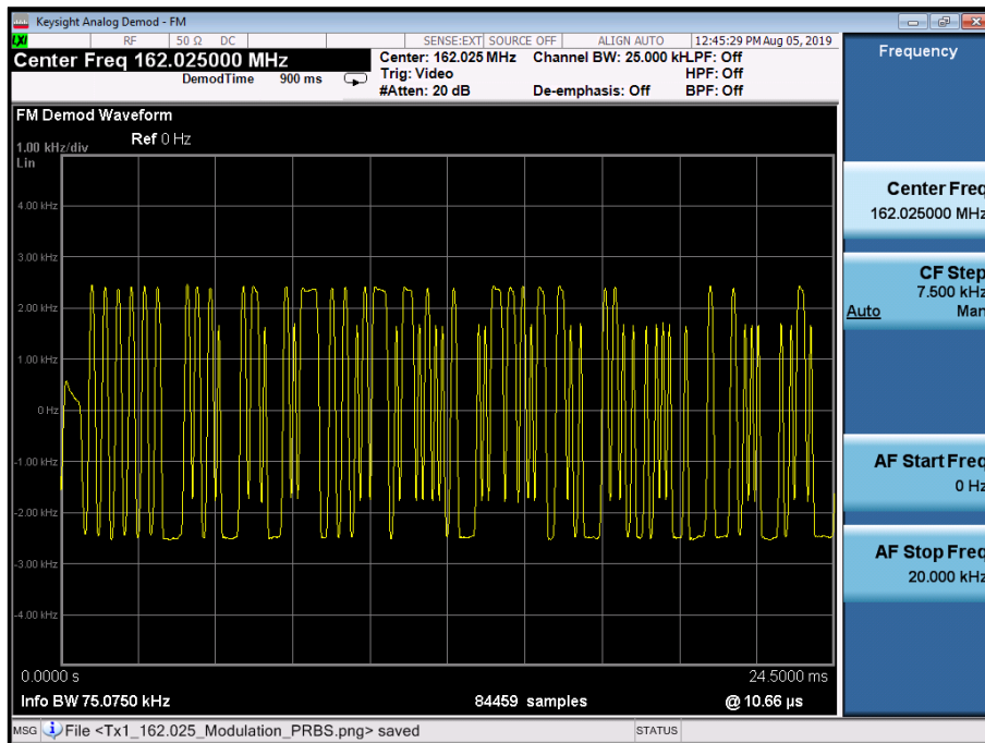
Figure 42- 162.025 MHz - PRBS
