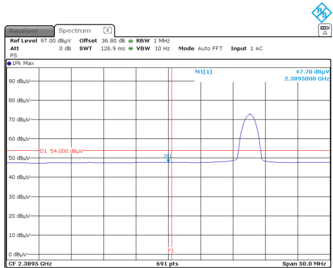
Figure 8.6-23: Radiated emissions in restricted Band 2390 MHz, Average Channel B
