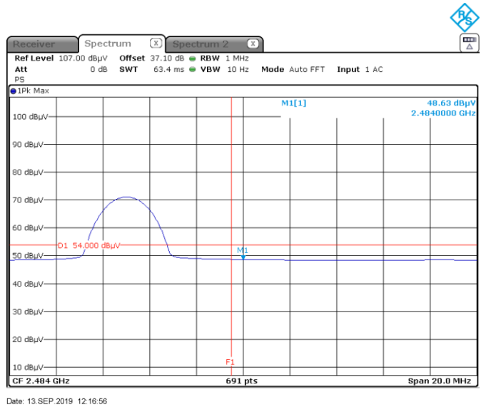
Figure 8.6-4: Radiated emissions in restricted Band 2483.5 MHz, Average Channel A
