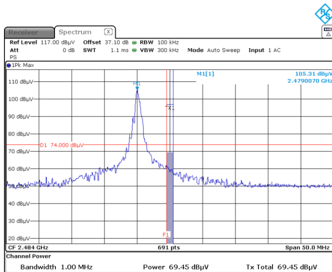
Figure 8.6-24: Radiated emissions in restricted Band 2483.5 MHz, Peak Channel B
