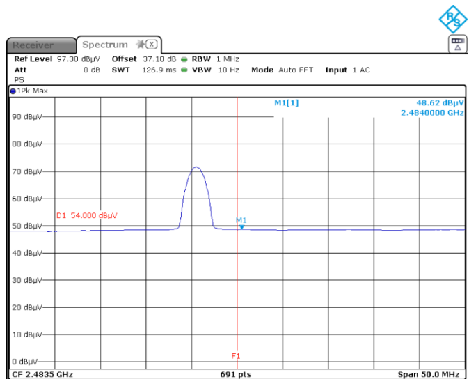
Figure 8.6-25: Radiated emissions in restricted Band 2483.5 MHz, Average Channel B
