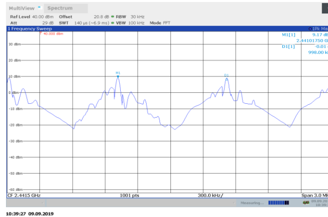
Figure 8.4-4: Carrier frequency separation, Channel A
