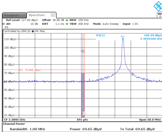
Figure 8.6-22: Radiated emissions in restricted Band 2390 MHz, Peak Channel B
