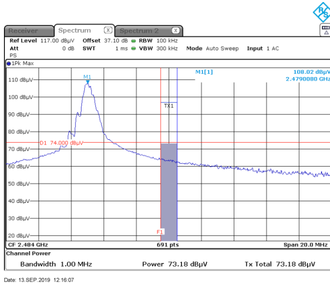
Figure 8.6-3: Radiated emissions in restricted Band 2483.5 MHz, Peak Channel A
