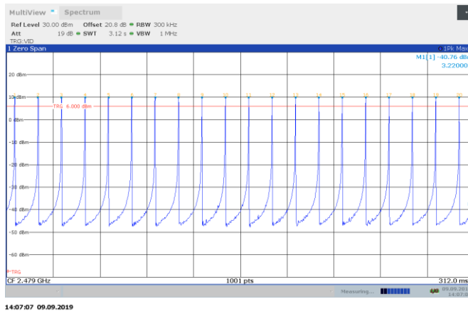
Figure 8.4-6: Average time of occupancy
