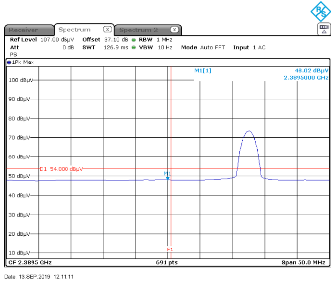
Figure 8.6-2: Radiated emissions in restricted Band 2390 MHz, Average Channel A
