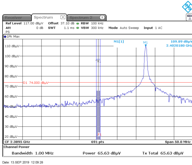
Figure 8.6-1: Radiated emissions in restricted Band 2390 MHz, Peak Channel A
