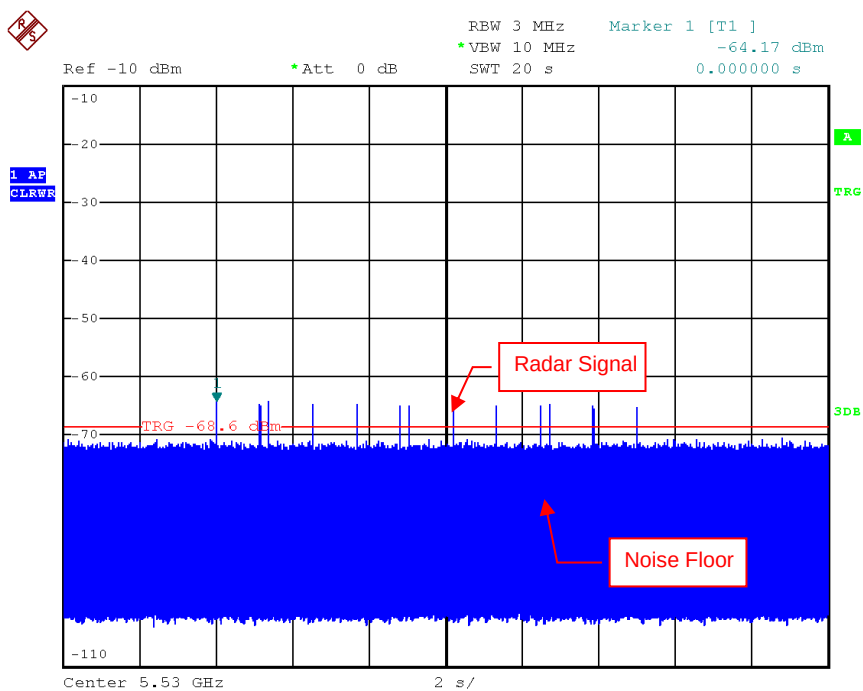
Radar Signal 5
