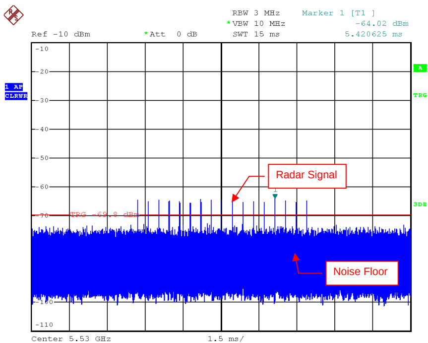
Radar Signal 3
