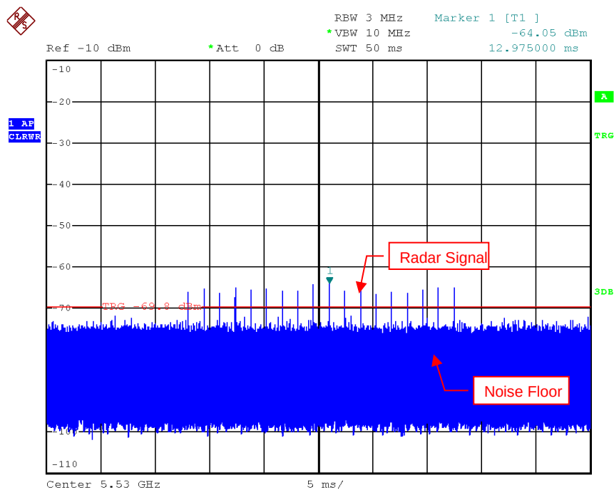
Radar Signal 0
