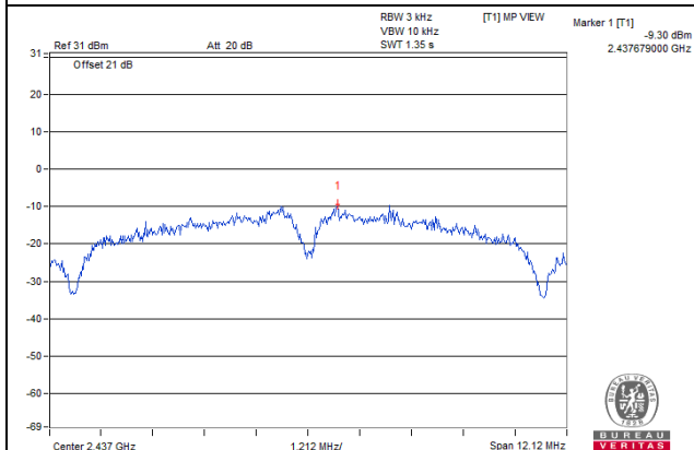
VHT20_Chain 0 / CH6
