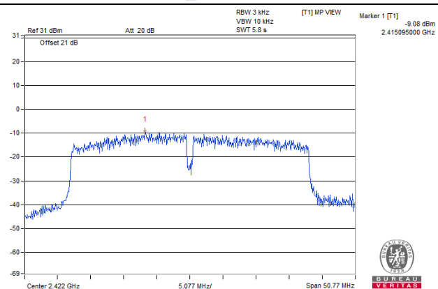
VHT40_Chain 1 / CH3
