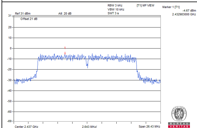
VHT20_Chain 0 / CH6
