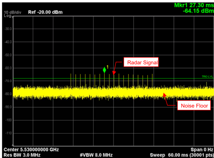
Radar Signal 0
