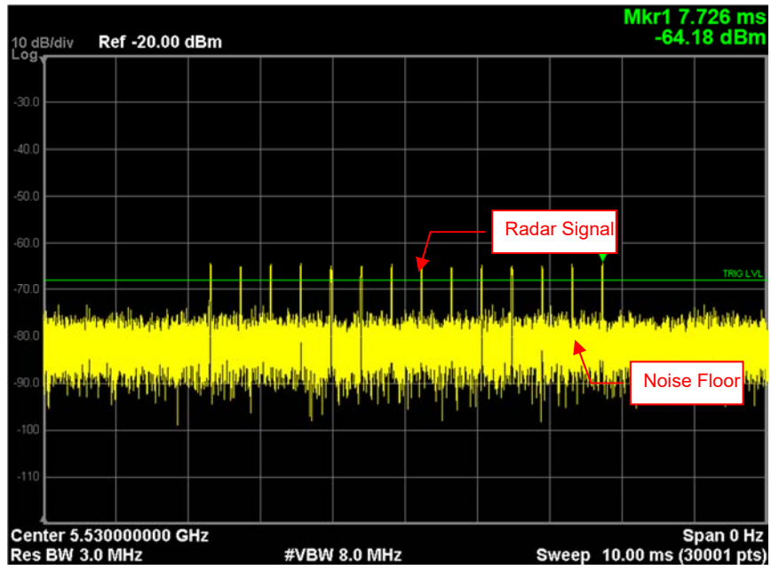
Radar Signal 2
