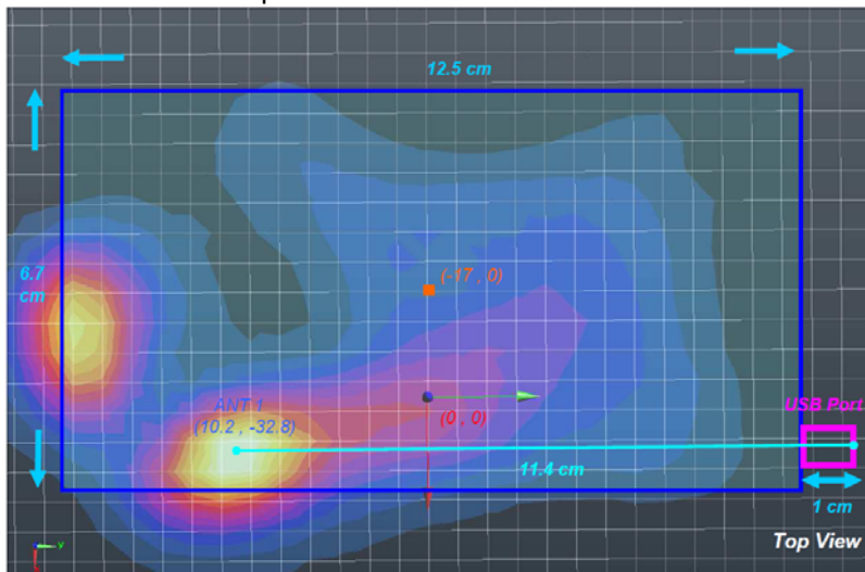
WiFi antenna 2 test plot
