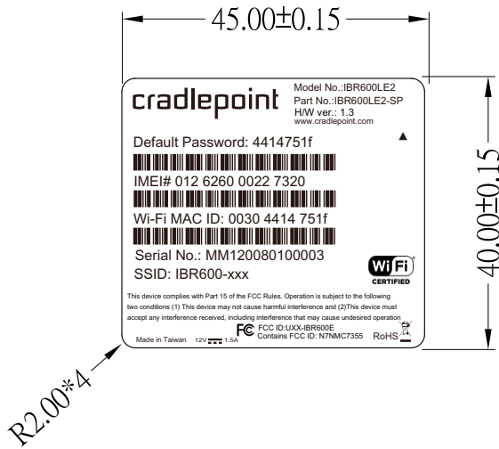
Bottom-Label for IBR600LE2-SP
