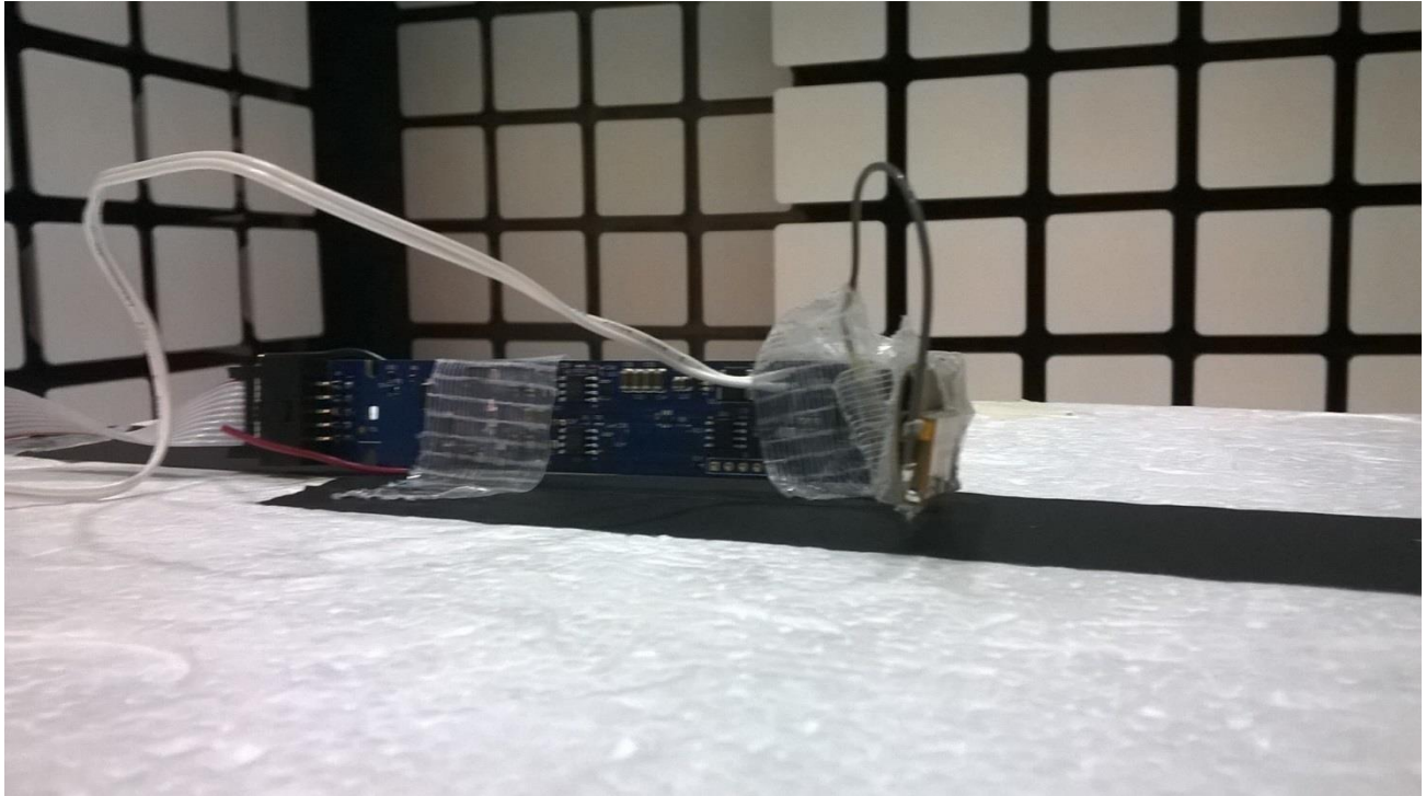
Figure 5 - Radiated Emissions Test Setup, Y axis (alternate view)
