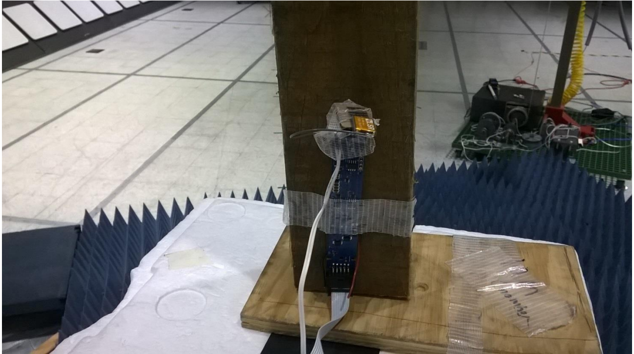
Figure 6 - Radiated Emissions Test Setup, Y axis
