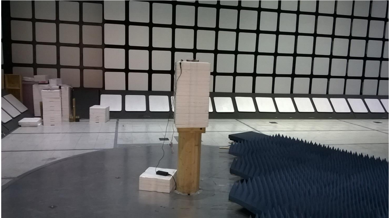
Figure 2 - Radiated Emissions Test Setup, 1 - 25 GHz
