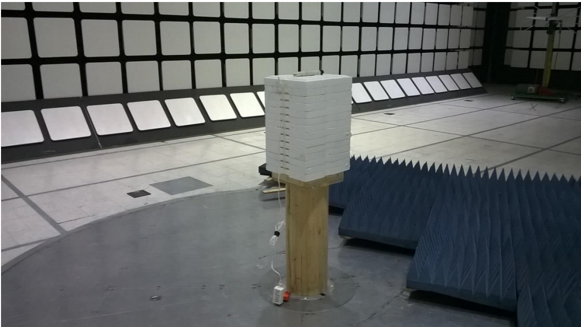
Figure 2 - Radiated Emissions Test Setup
