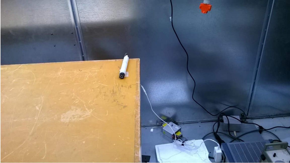
Figure 3 - Conducted Emissions Test Setup
