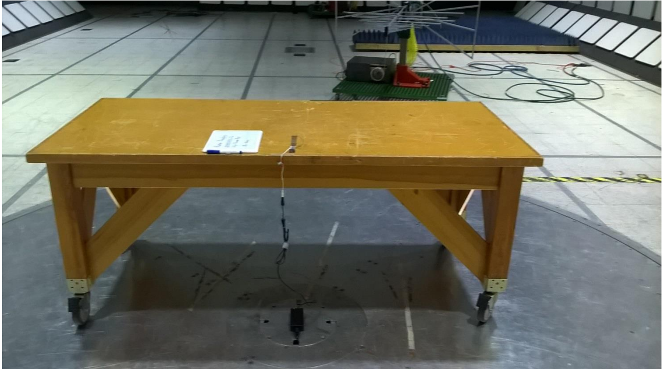
Figure 1 - Radiated Emissions Test Setup, 30MHz - 1GHz
