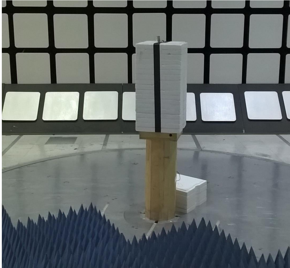
Figure 2 - Radiated Emissions Test Setup, 1 - 25 GHz
