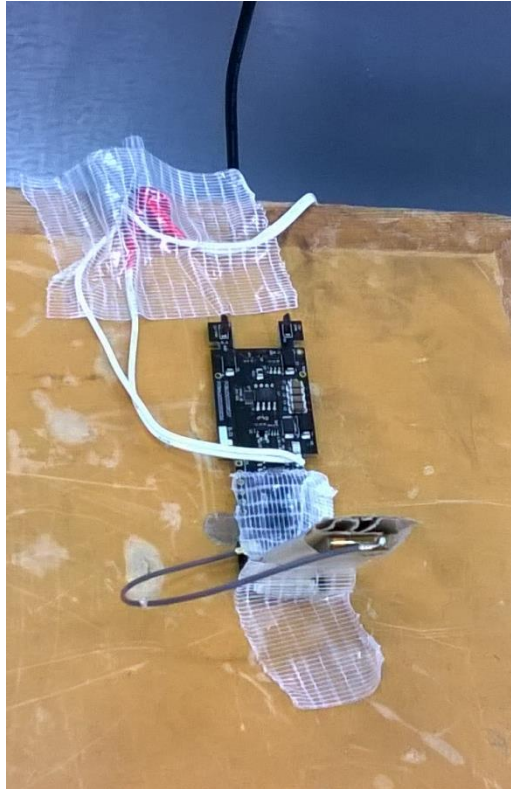
Figure 7 – Conducted Emissions Test Setup
