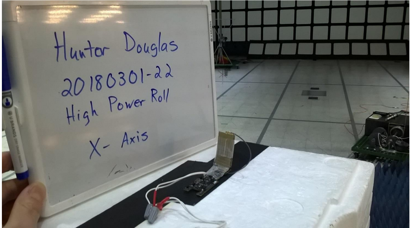
Figure 3 - Radiated Emissions Test Setup, X axis
