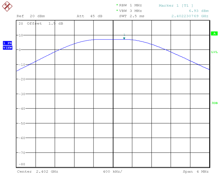
Figure 3: Maximum Conducted Power, 2402 MHz, 1Mbps
