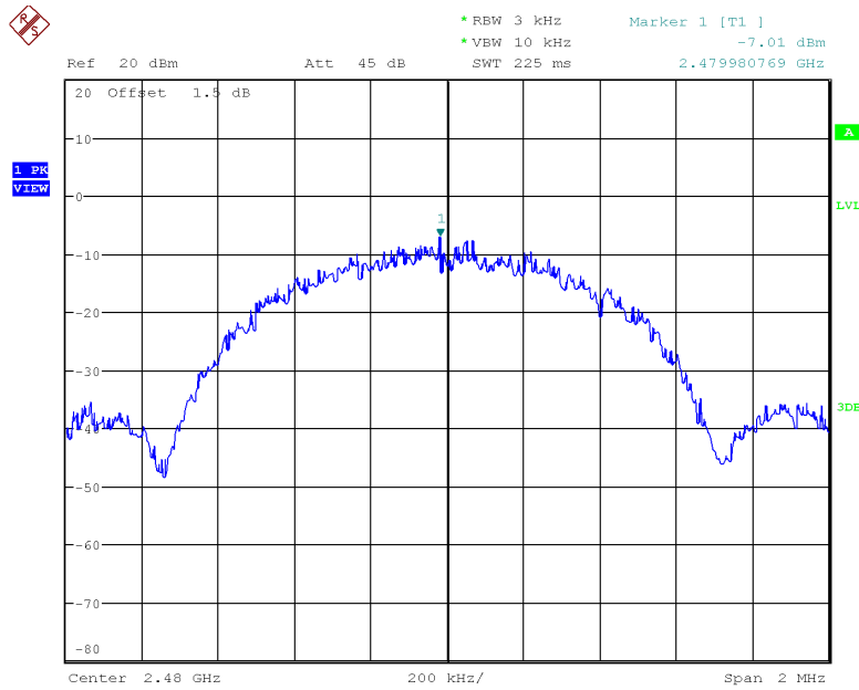
Figure 23: 2480MHz, 1Mbps, PSD
