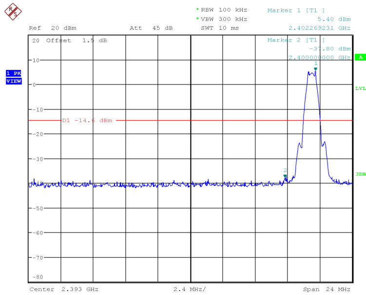
Figure 27: 2402MHz, 1Mbps, Lower Band Edge
