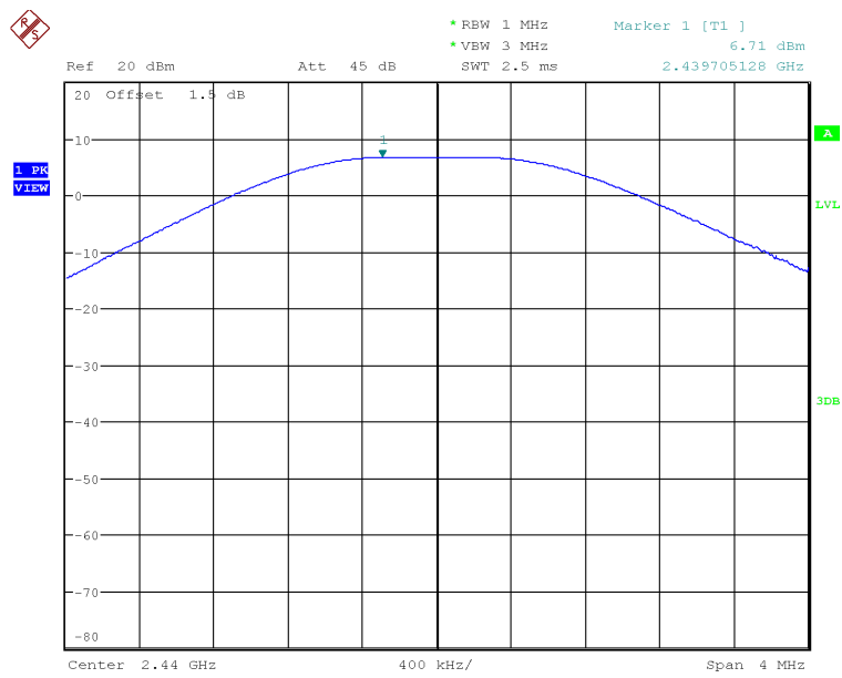
Figure 4: Maximum Conducted Power, 2440MHz, 1Mbps
