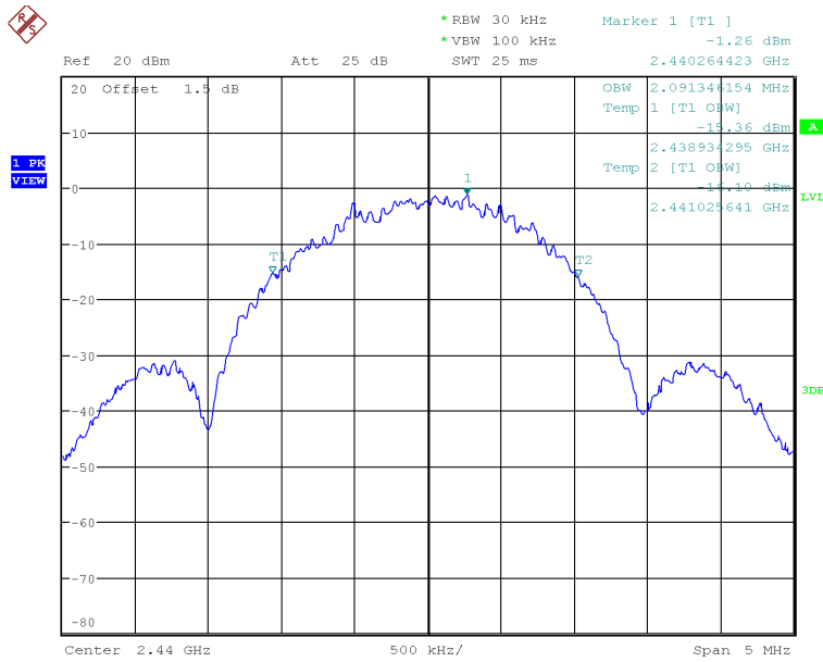
Figure 19: 2440MHz, 2Mbps, 99% Bandwidth
