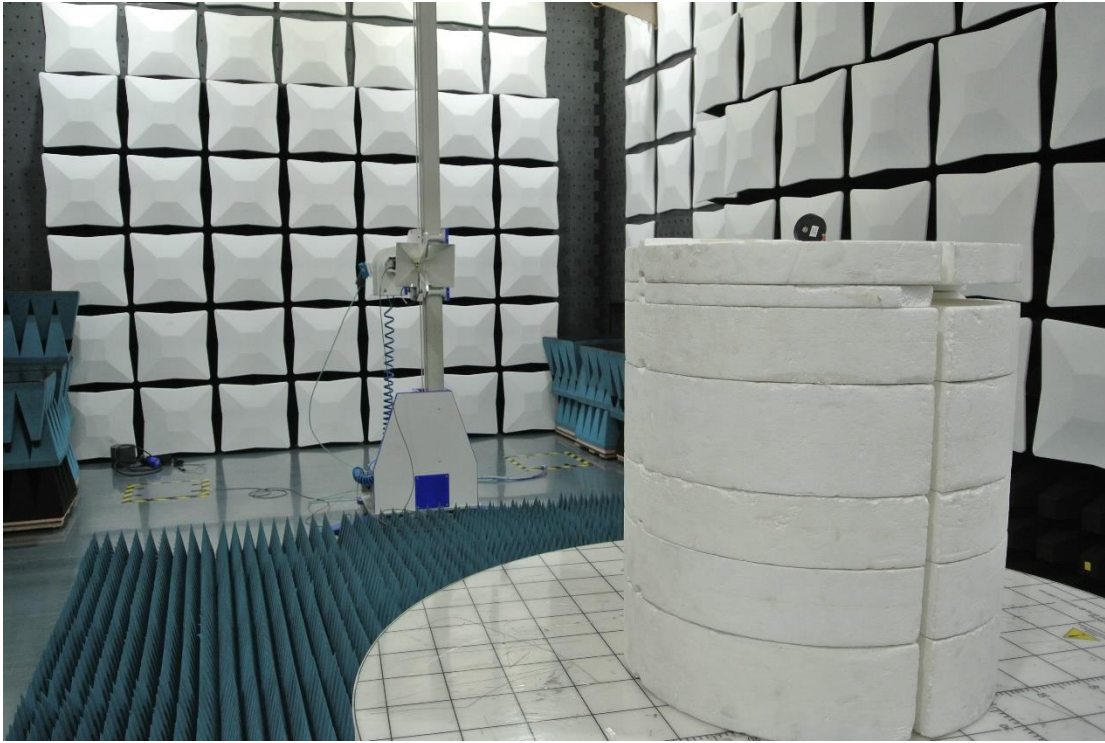
Figure 4: Test Setup for 1 GHz to 18 GHz (View 2)
