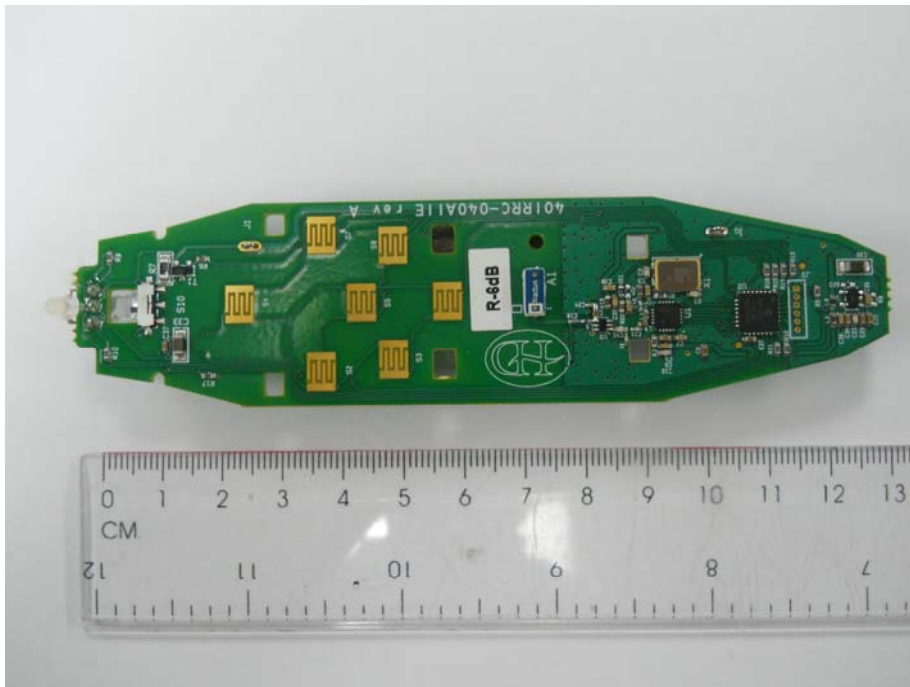
Top View (Main PCB)
