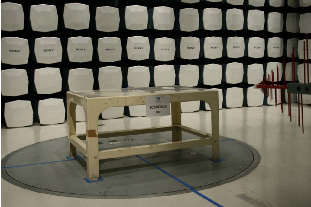
Radiated Emissions Test Setup (Below 1GHz)
