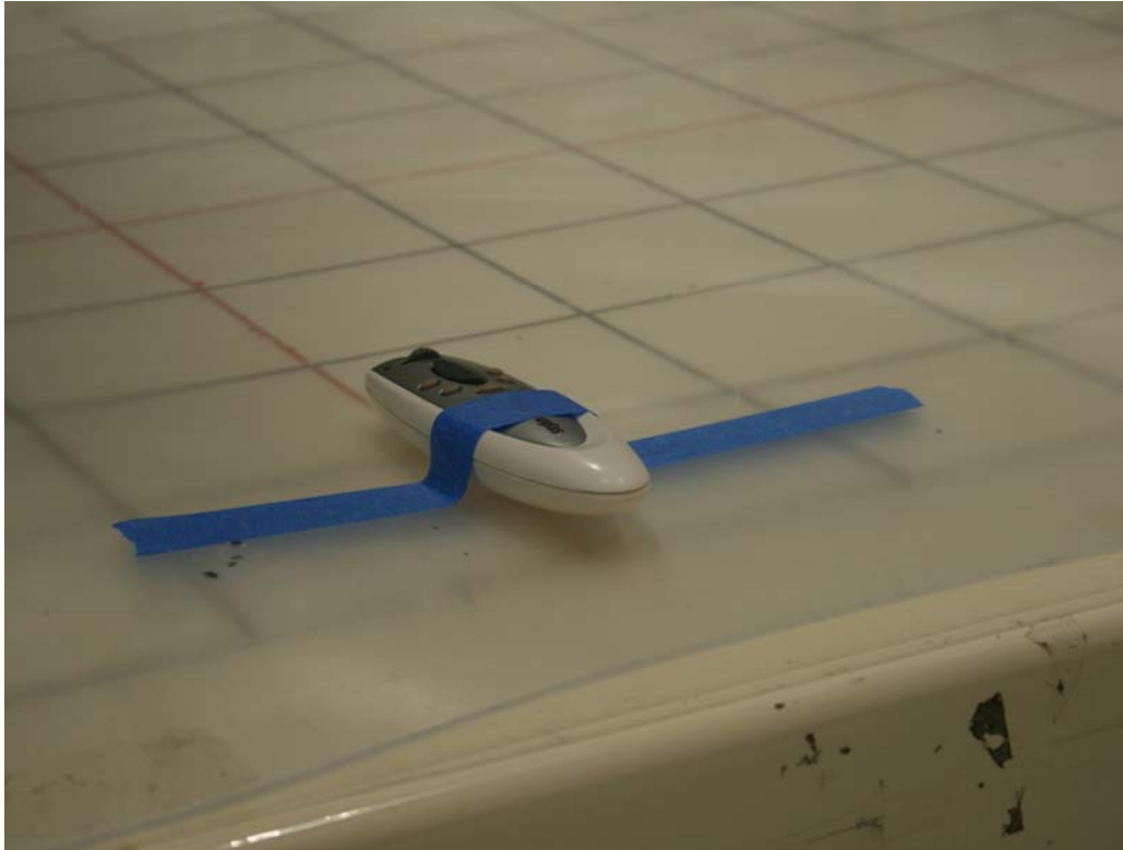
Radiated Emissions Test Setup (X axis configuration)
