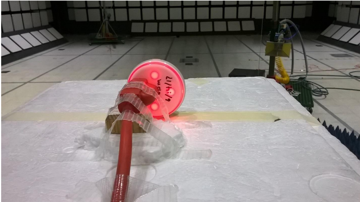
Figure 3 - EUT Test Setup – X-axis
