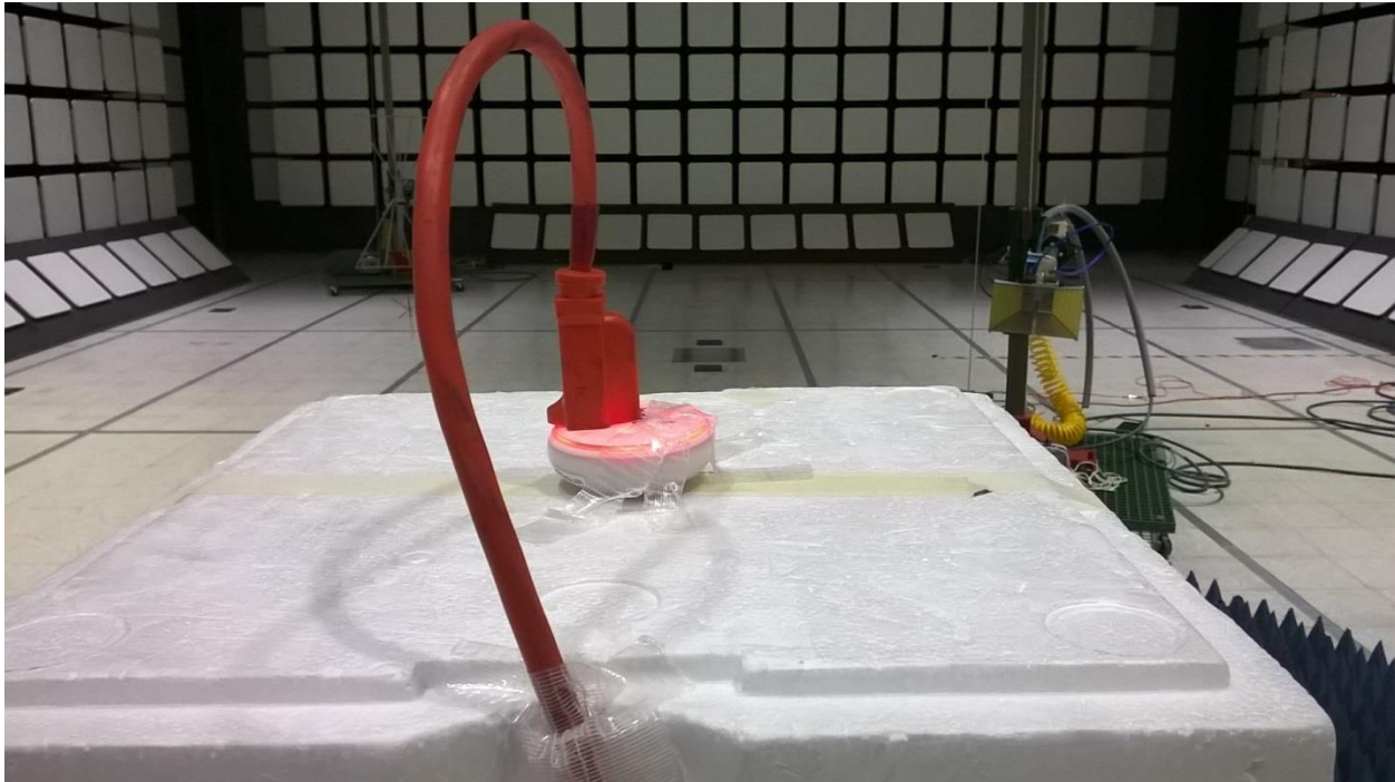
Figure 4 - EUT Test Setup – Y-axis
