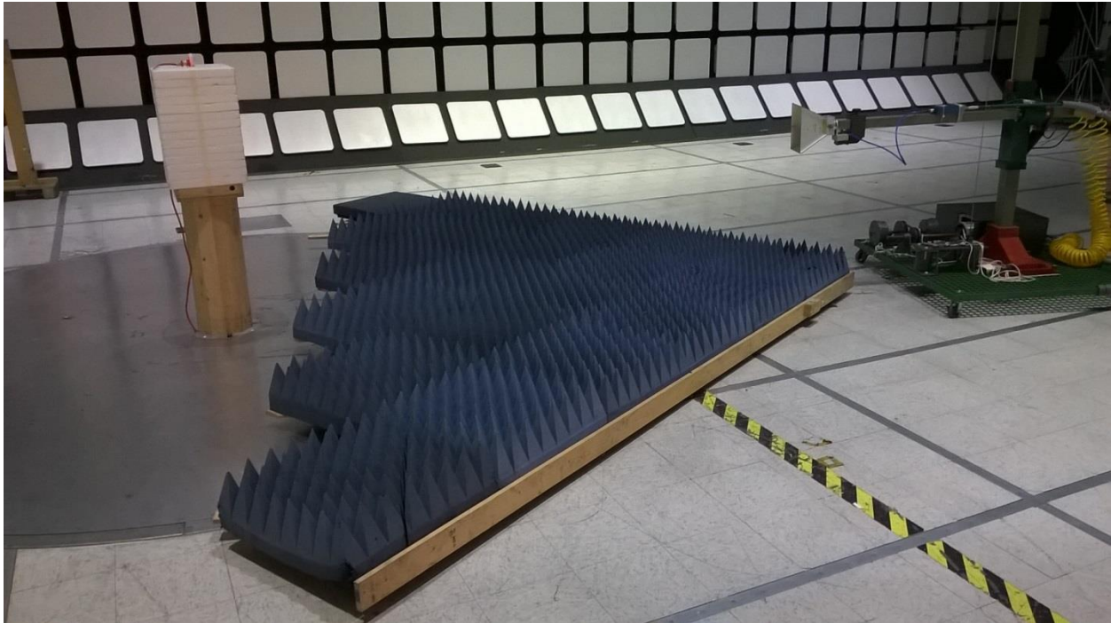
Figure 1 - EUT Test Setup, 1GHz – 25GHz
