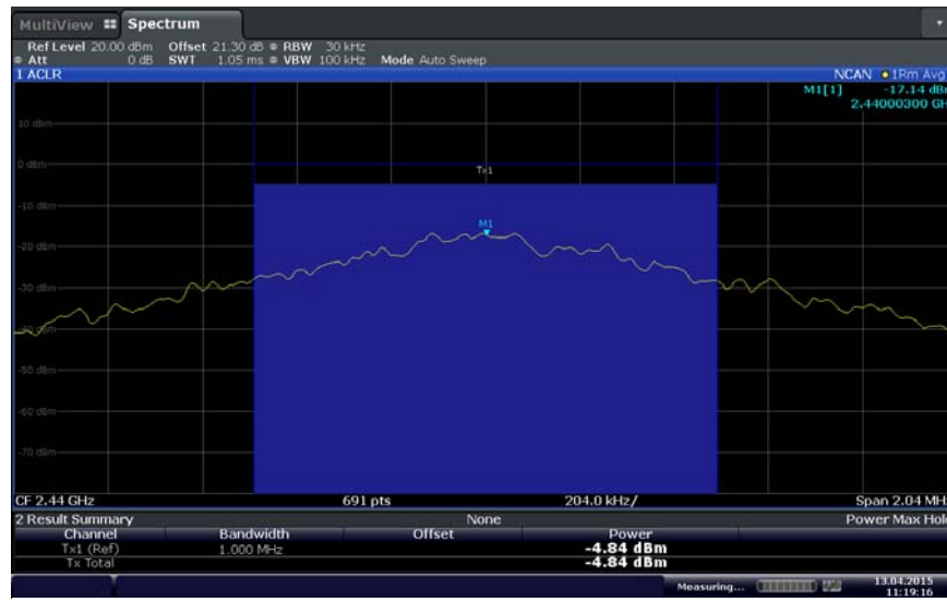
Mid Channel (2440 MHz)
