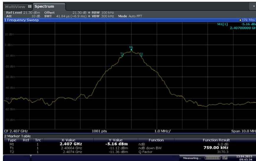
Low Channel (2407 MHz)
