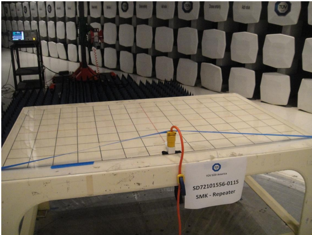
Radiated Emission Measurement Above 1GHz (Front and rear)
