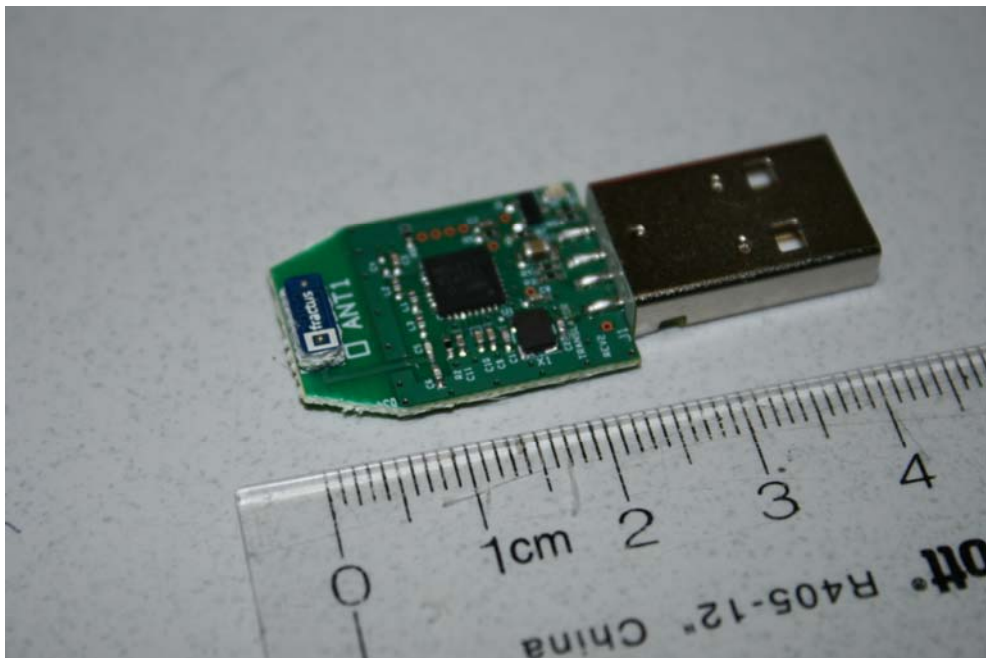
Top View (Main PCB)
