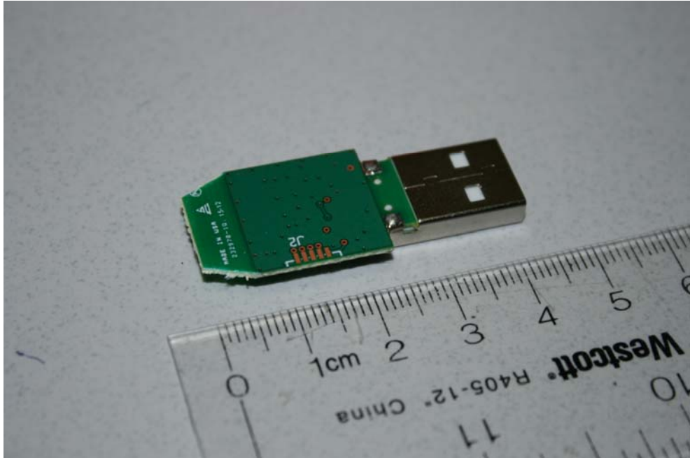
Bottom View (Main PCB)
