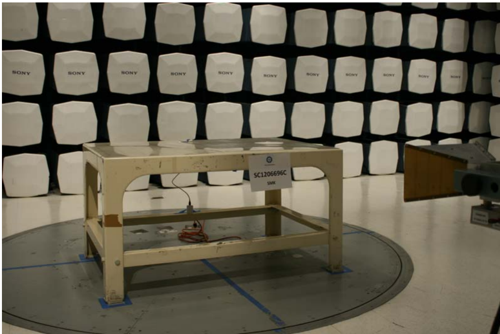
Radiated Emissions Test Setup (Above 1GHz)
