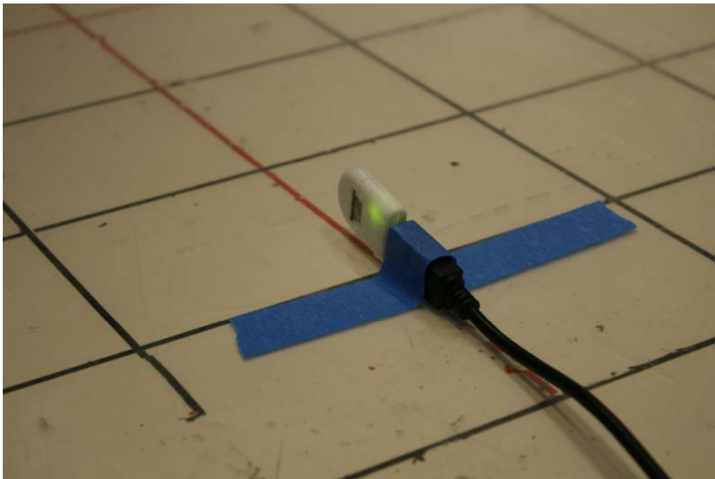
Radiated Emissions Test Setup (Y axis configuration)
