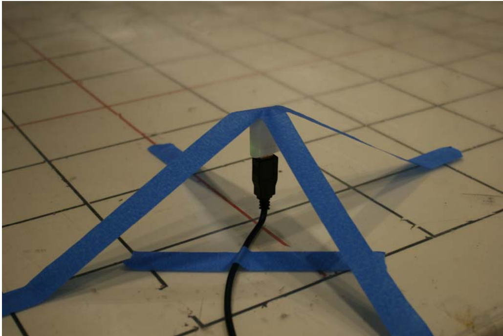
Radiated Emissions Test Setup (Z axis configuration)
