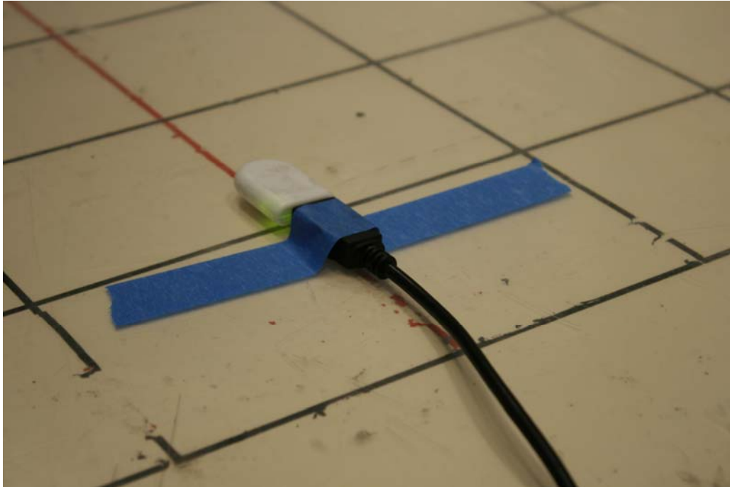
Radiated Emissions Test Setup (X axis configuration)
