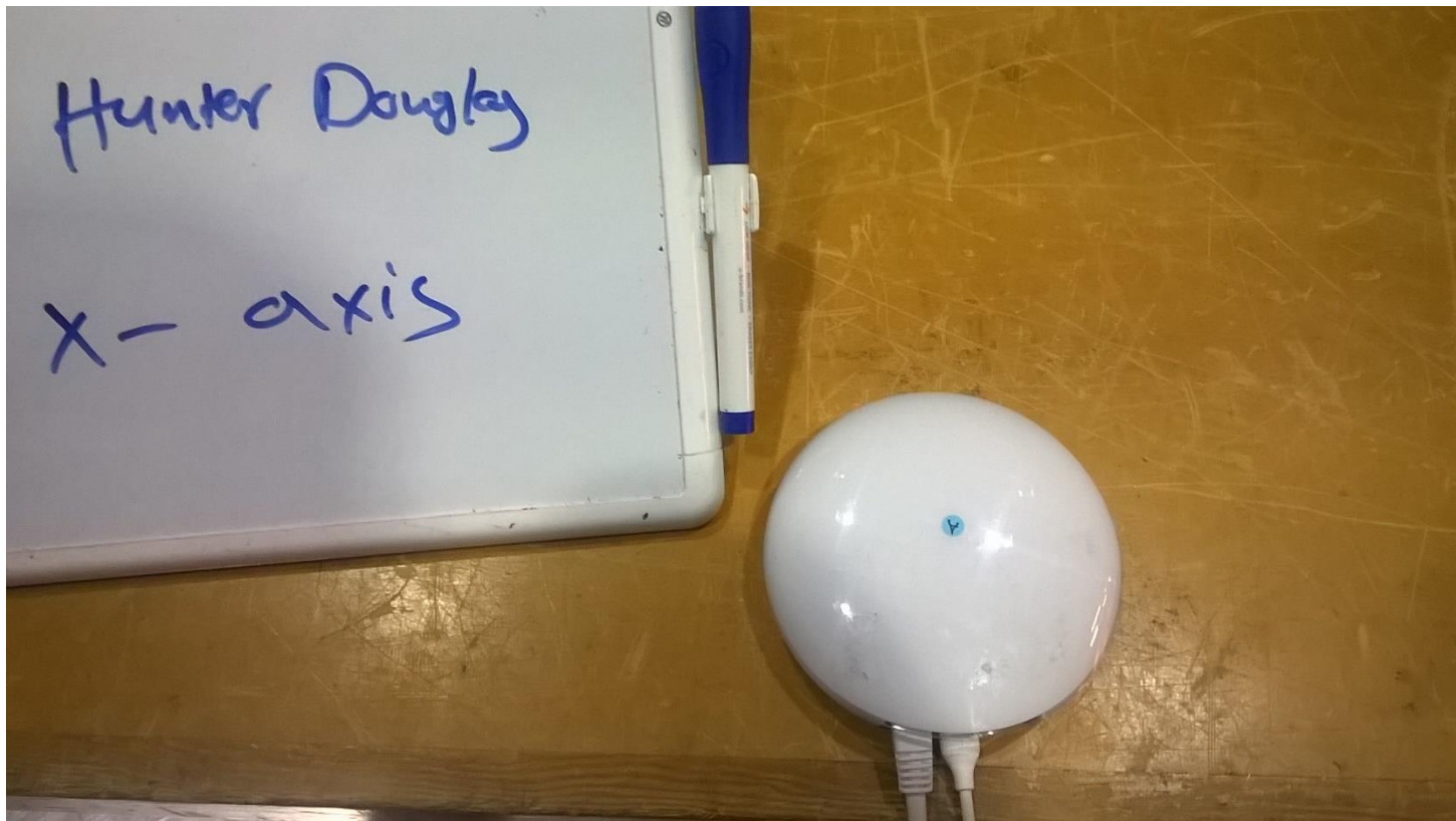
Figure 3 - Radiated Emissions Test Setup, X-axis
