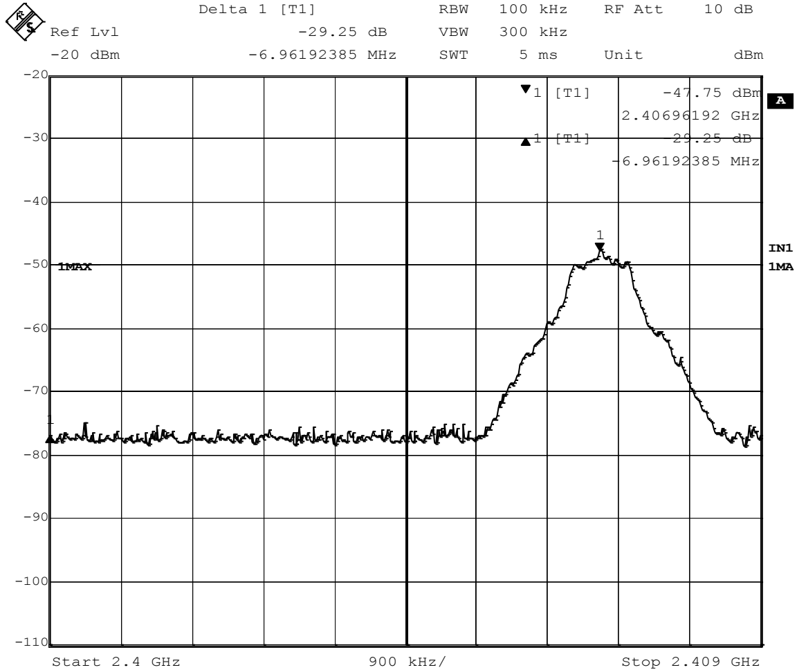
Figure 17 - Band-edge Measurement, Low Channel, out-of-band The plot shows an uncorrected measurement, used for relative measurements only.
