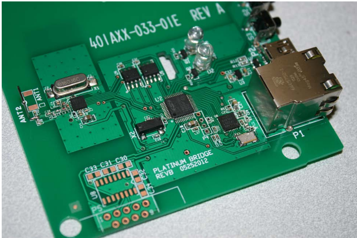
Top View (Main PCB with magnetic sheet removed)
