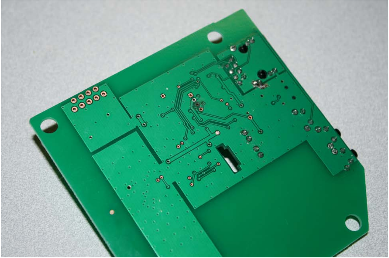
Bottom View (Main PCB with magnetic sheet removed )
