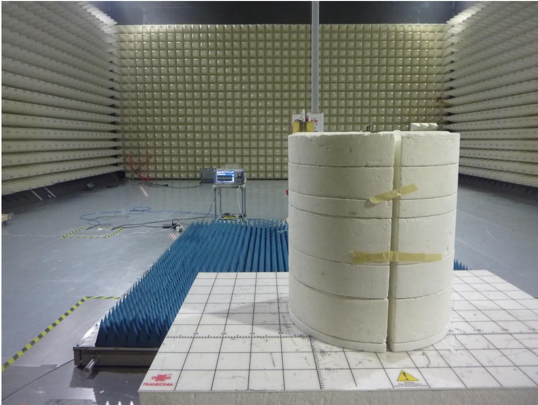
Figure 4: Test Setup for 1 GHz to 18 GHz (View 2)
