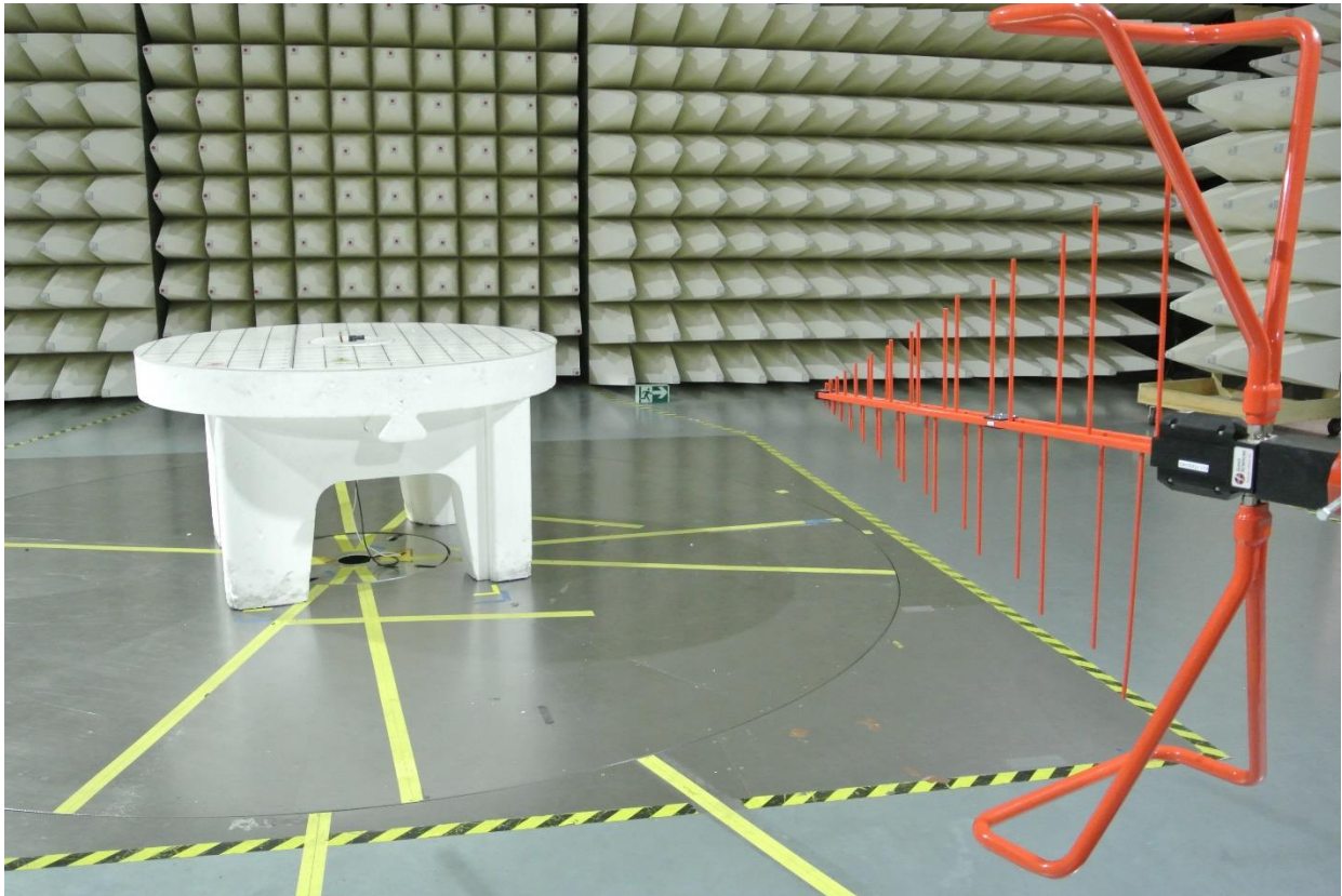
Figure 1: Test Setup for 30 MHz to 1 GHz (View 1)
