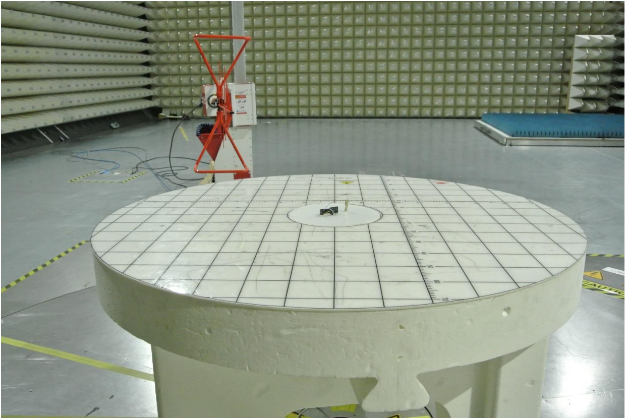
Figure 2: Test Setup for 30 MHz to 1 GHz (View 2)
