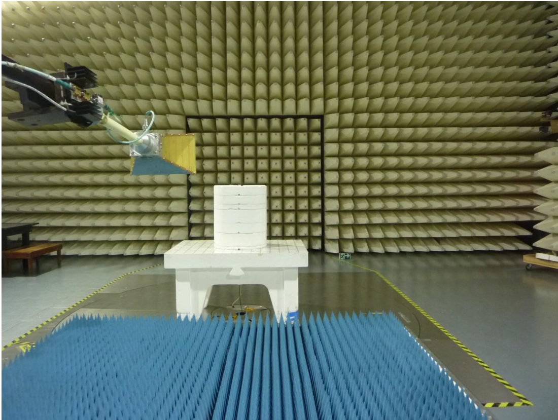
Figure 3: Test Setup for 1 GHz to 18 GHz (View 1)
