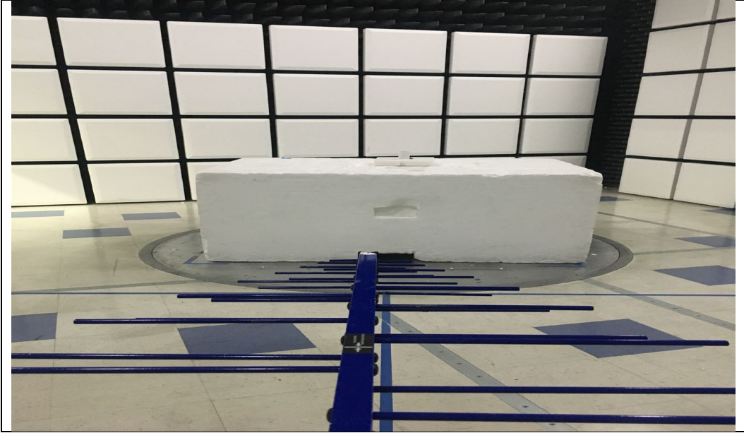
RF Radiated 30 MHz-1GHz
