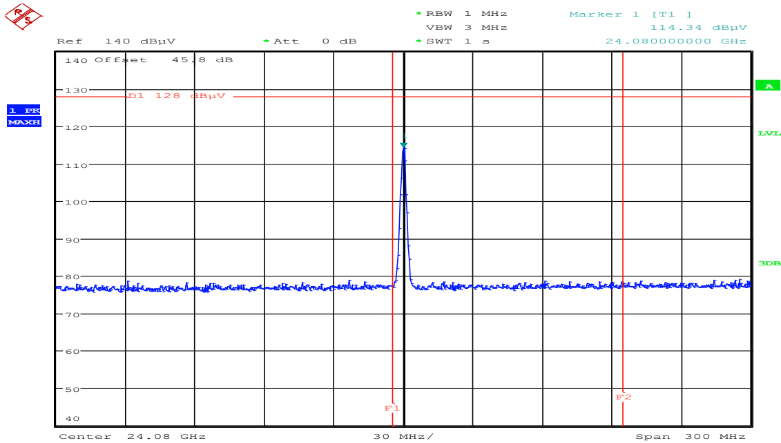
Plot 2: Field strength, peak measurement
