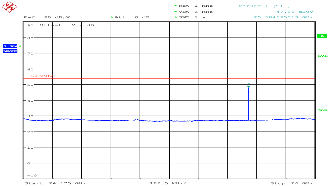
Plot 10: 24.175 GHz to 26 GHz
