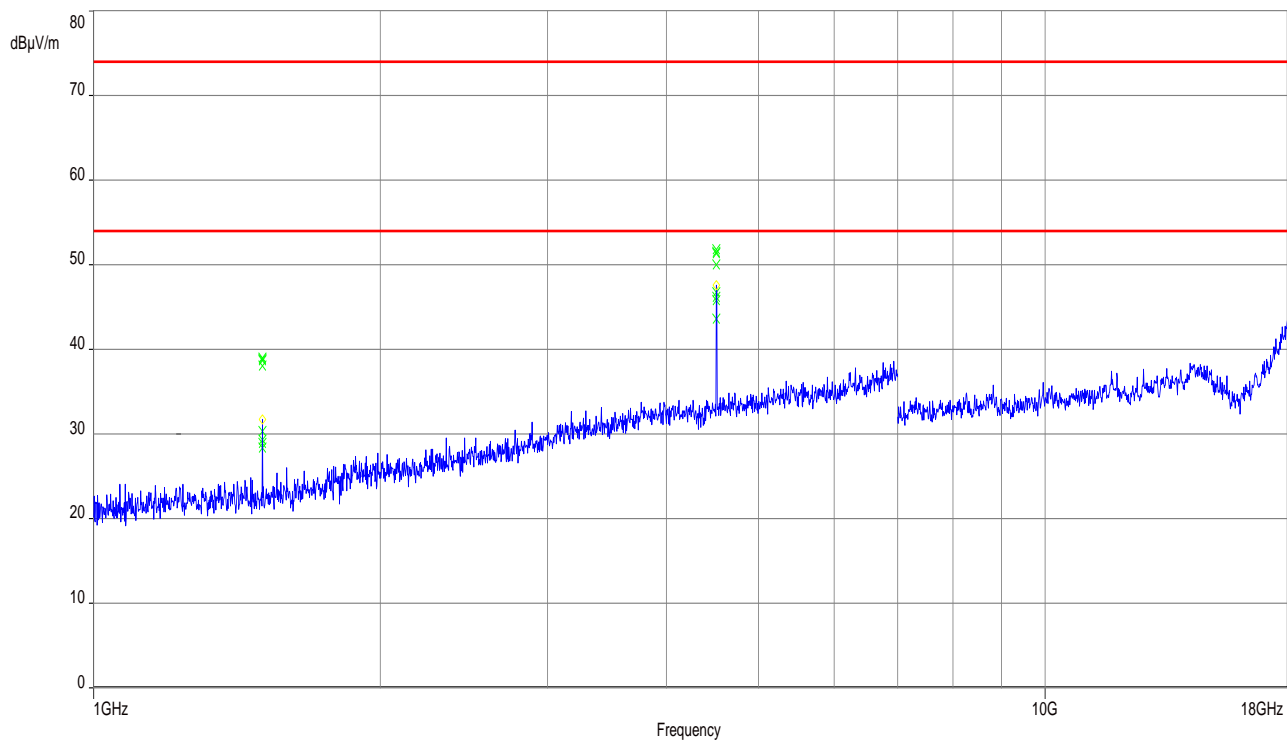
Plot 6: 1 GHz to 18 GHz, horizontal / vertical polarization
