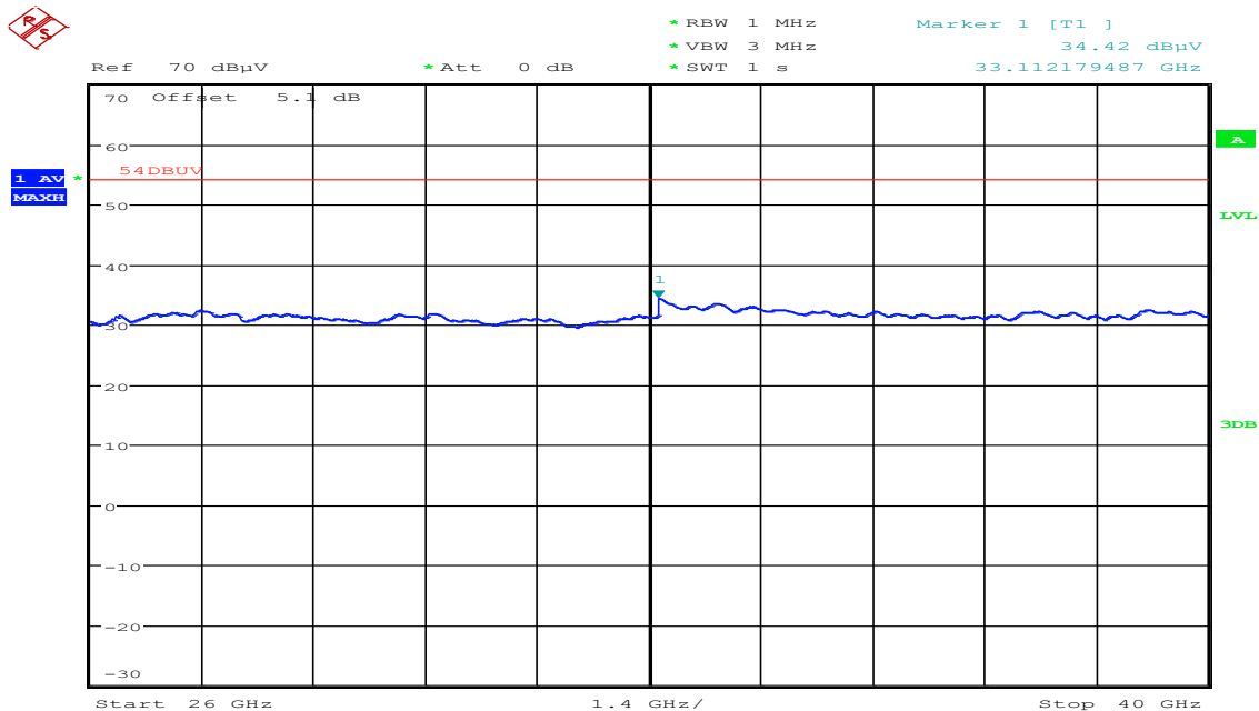
Plot 11: 26 GHz to 40 GHz
