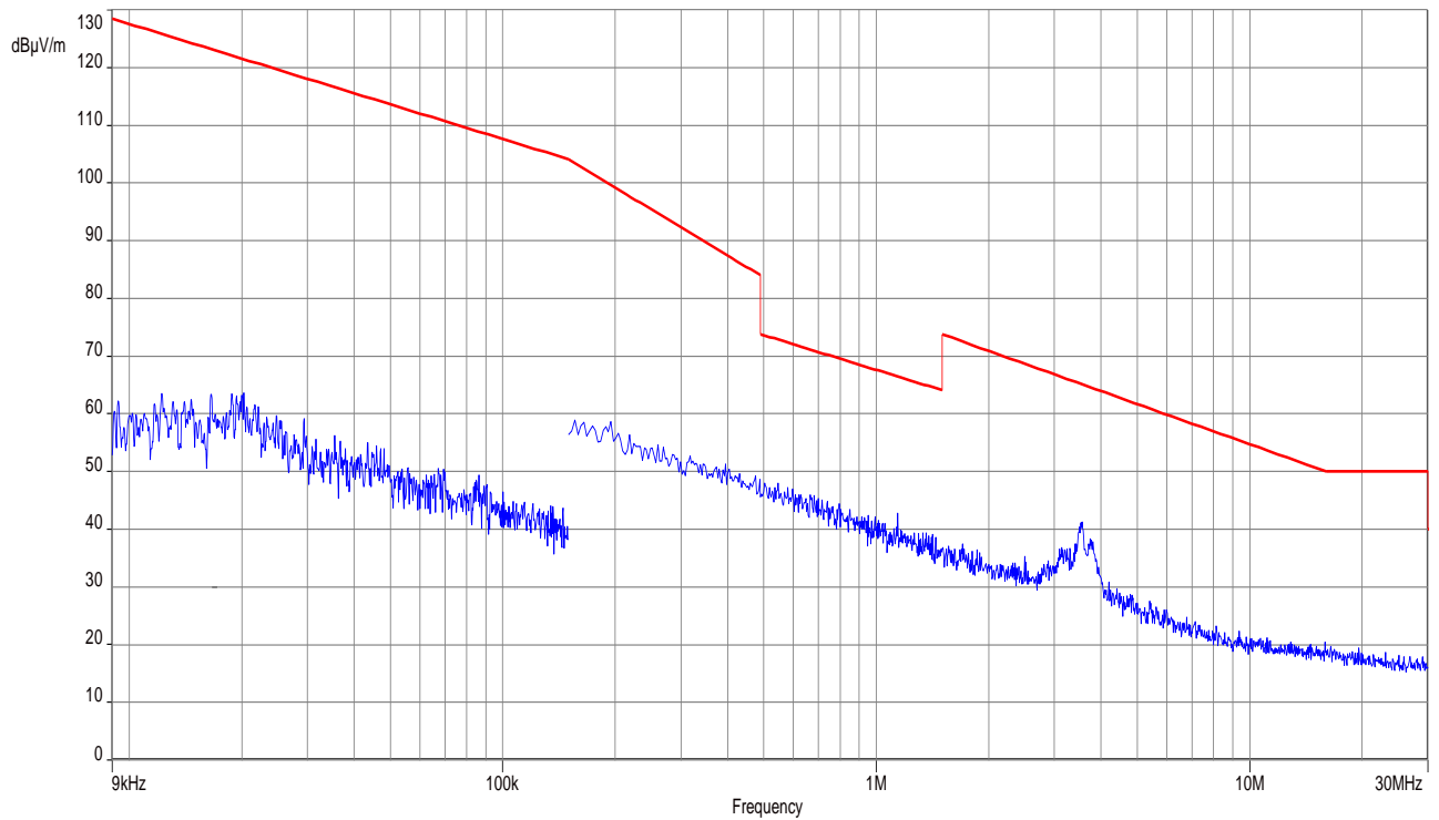
Plot 4: 9 kHz to 30 MHz, horizontal / vertical polarization
