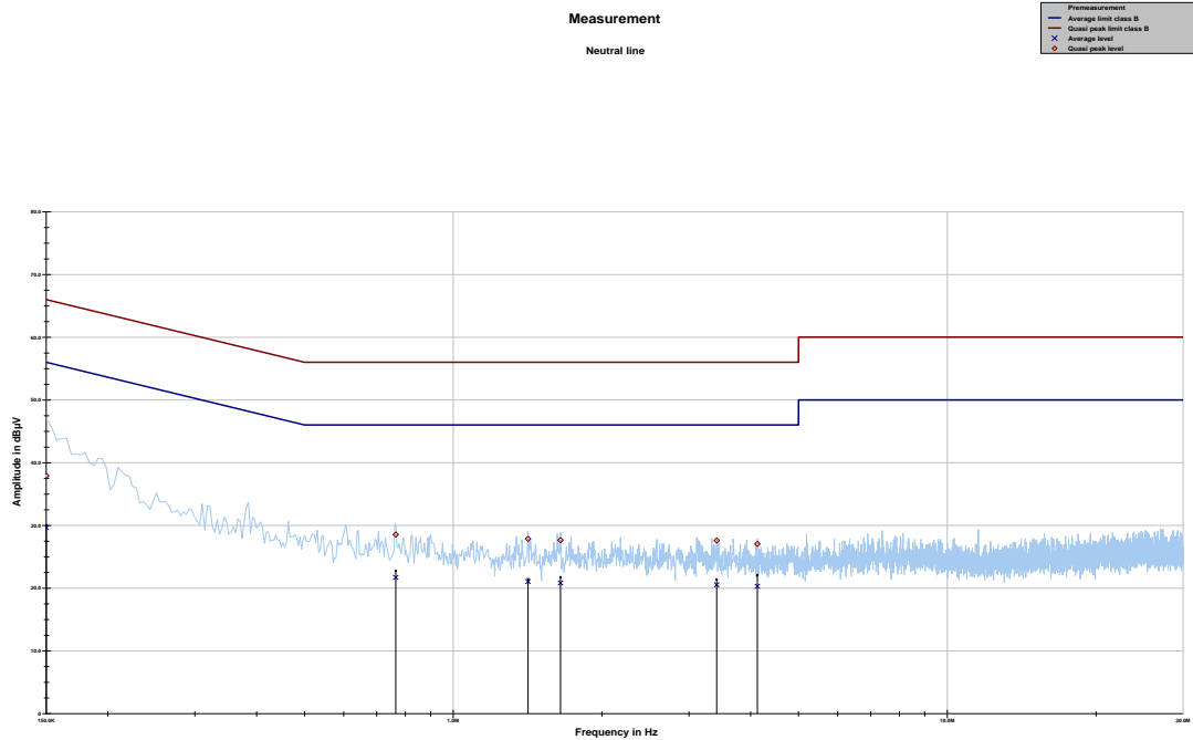
Plot 16: Neutral line
