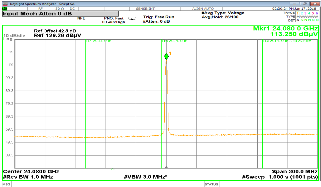
Plot 1: Field strength, RMS measurement
