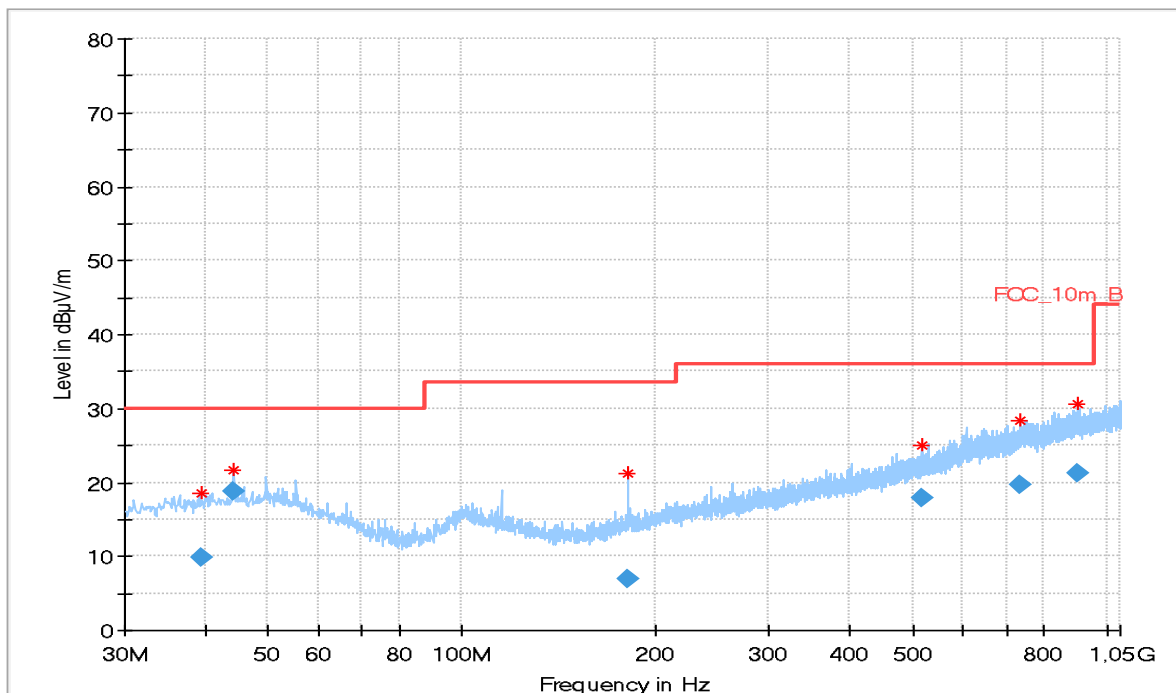
Plot 5: 30 MHz to 1 GHz, horizontal / vertical polarization
