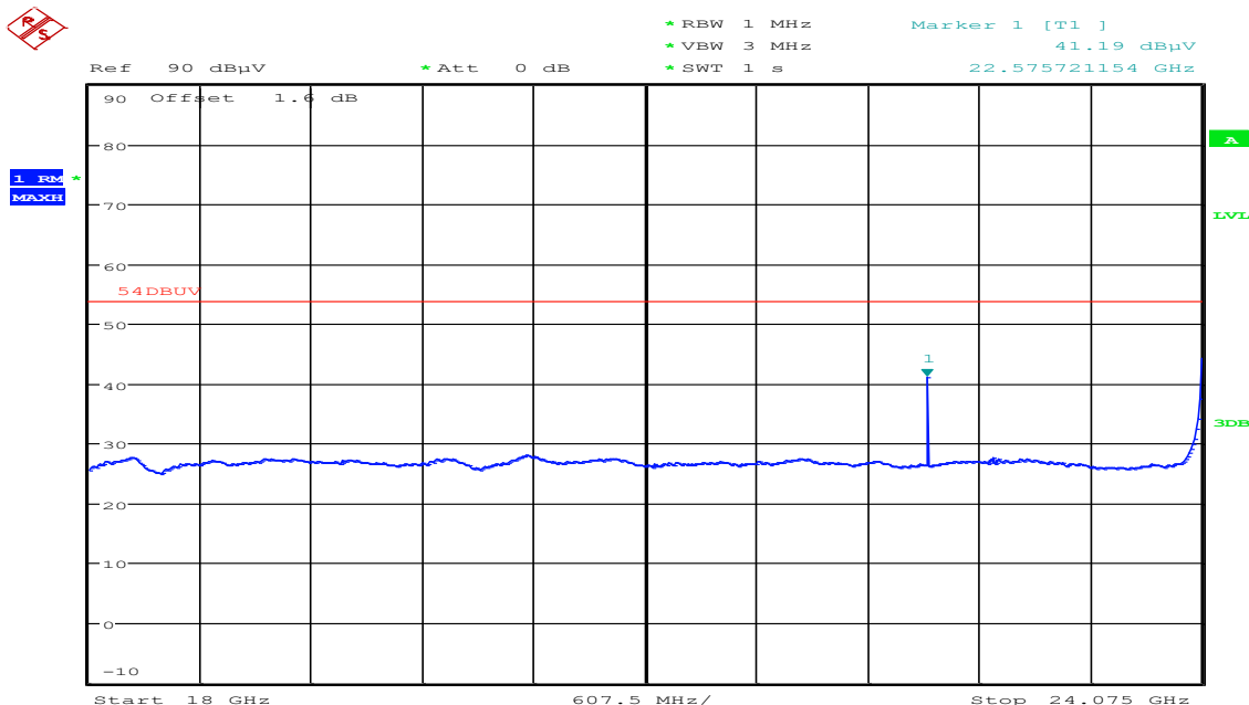
Plot 7: 18 GHz to 24.075 GHz
