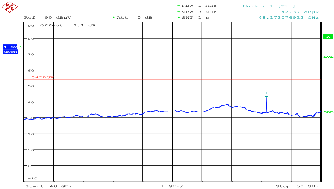
Plot 12: 40 GHz to 50 GHz
