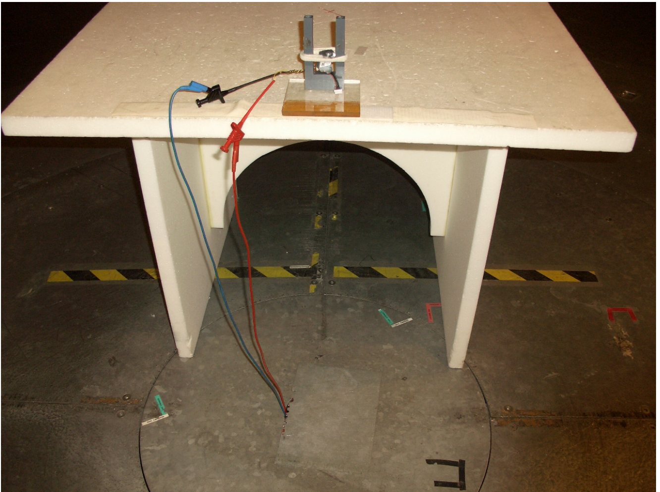
Spurious emission measurement 30 MHz – 1 GHz
