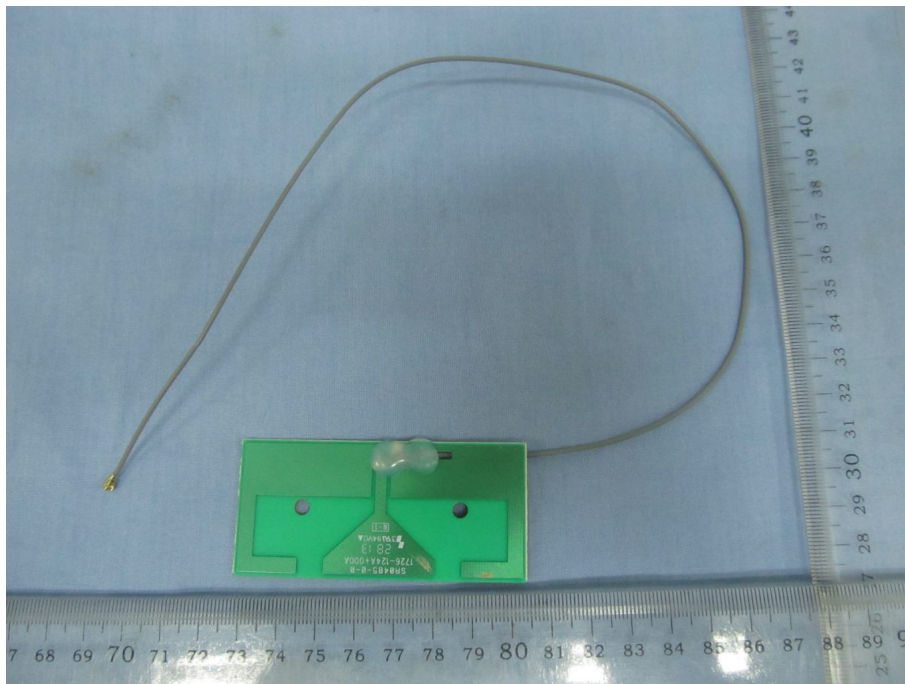
#1 antenna
