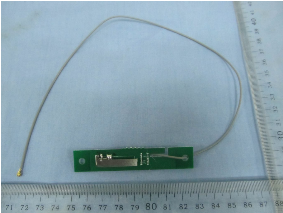
#2 antenna
